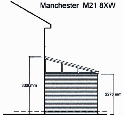
Proposed Side Section Elevation 1:100
