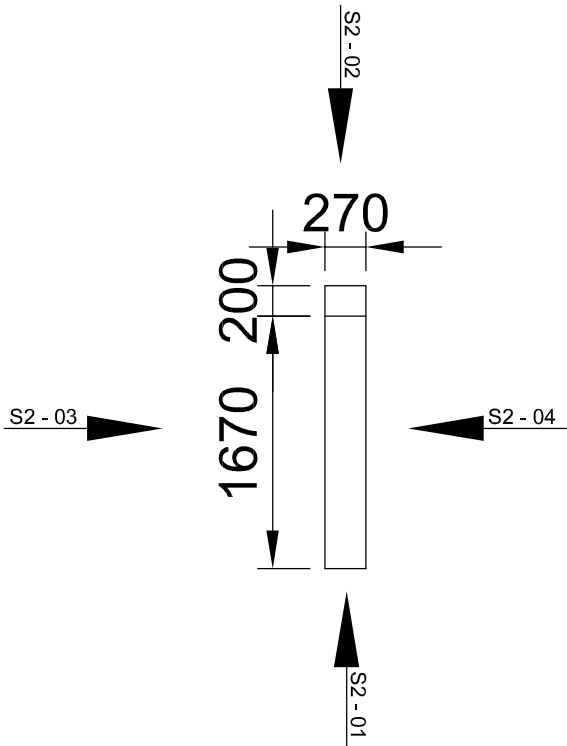
Sign S2 - plan
