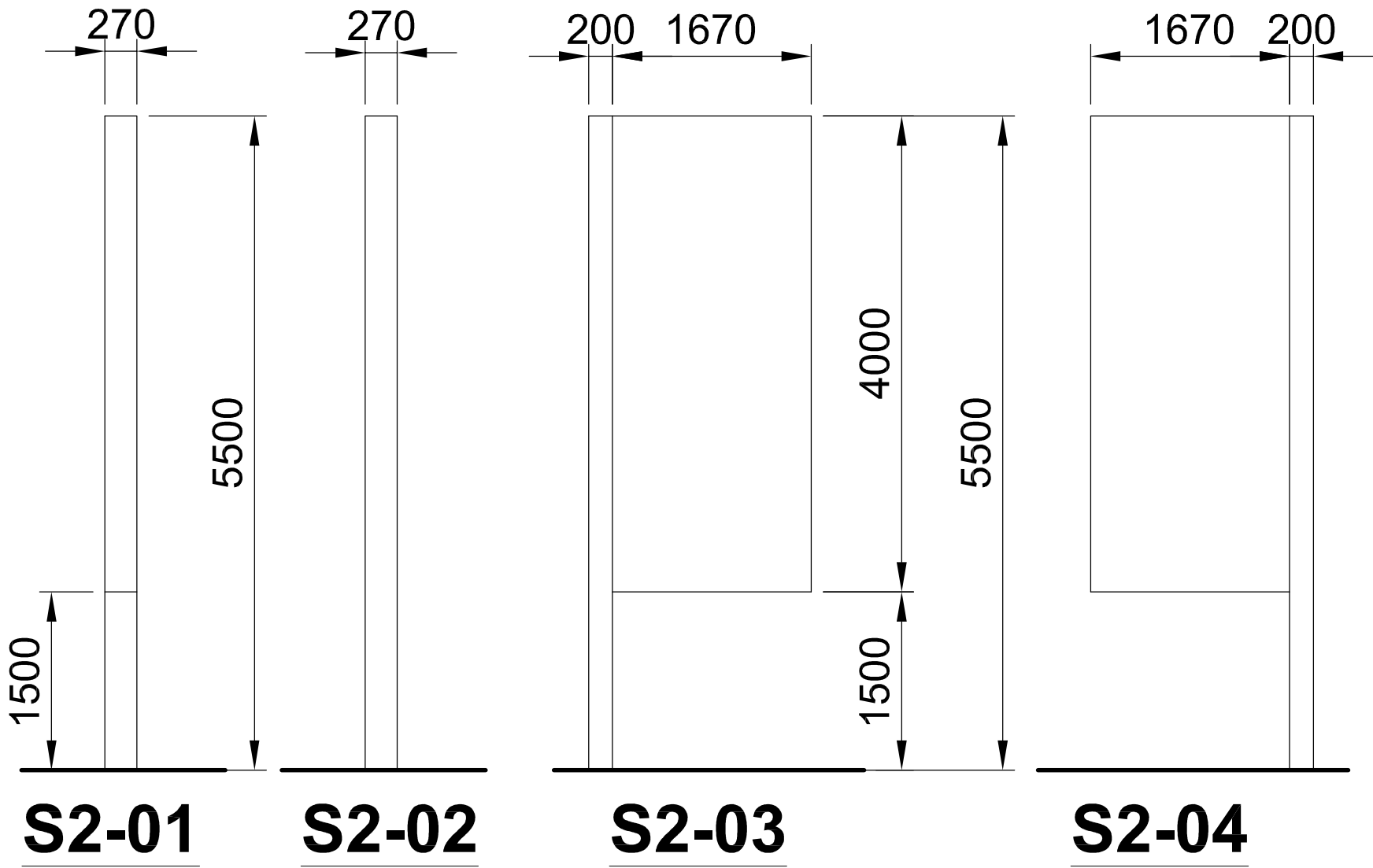
Sign S2 - elevations
