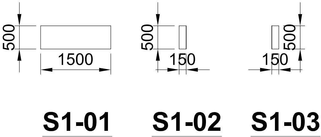
Sign S1 - elevations
