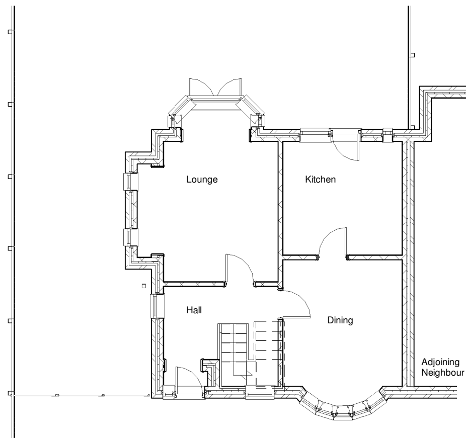
01 Existing Ground Floor Plan 1 : 100
