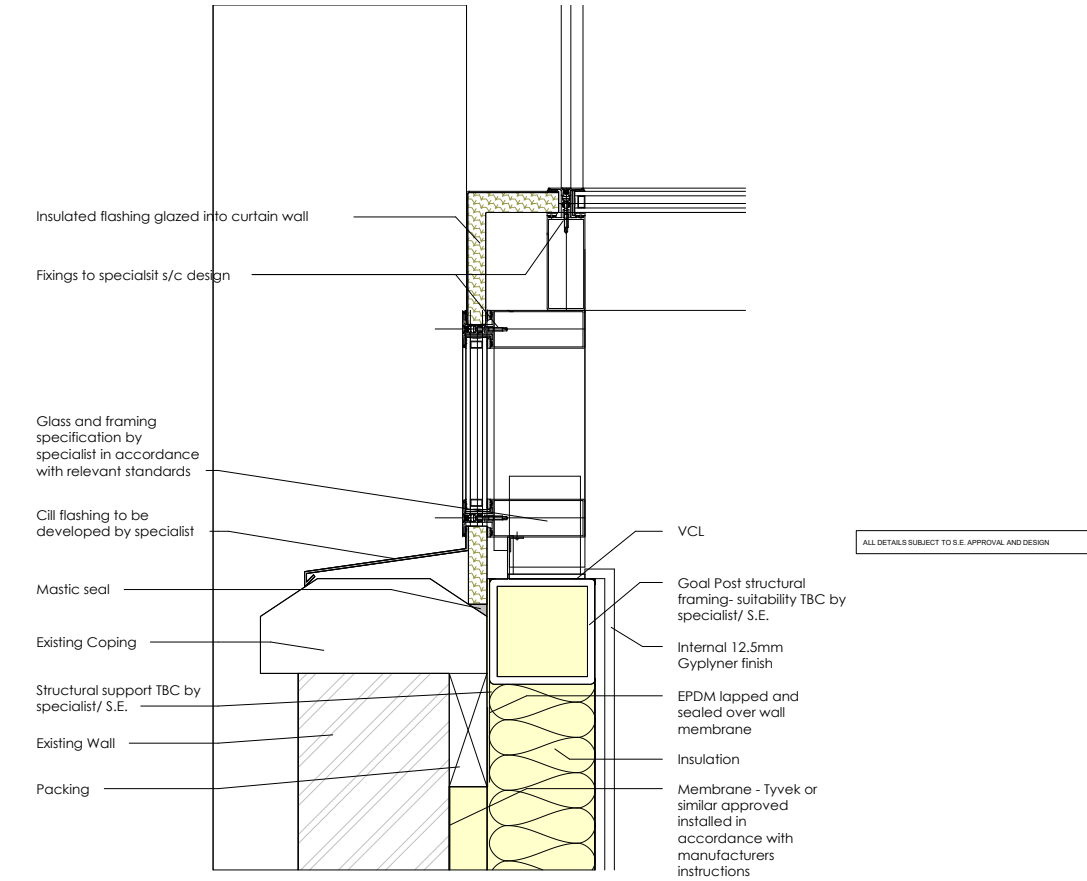
3 Garden Wall and Lean-To Junction Detail 1 : 10
