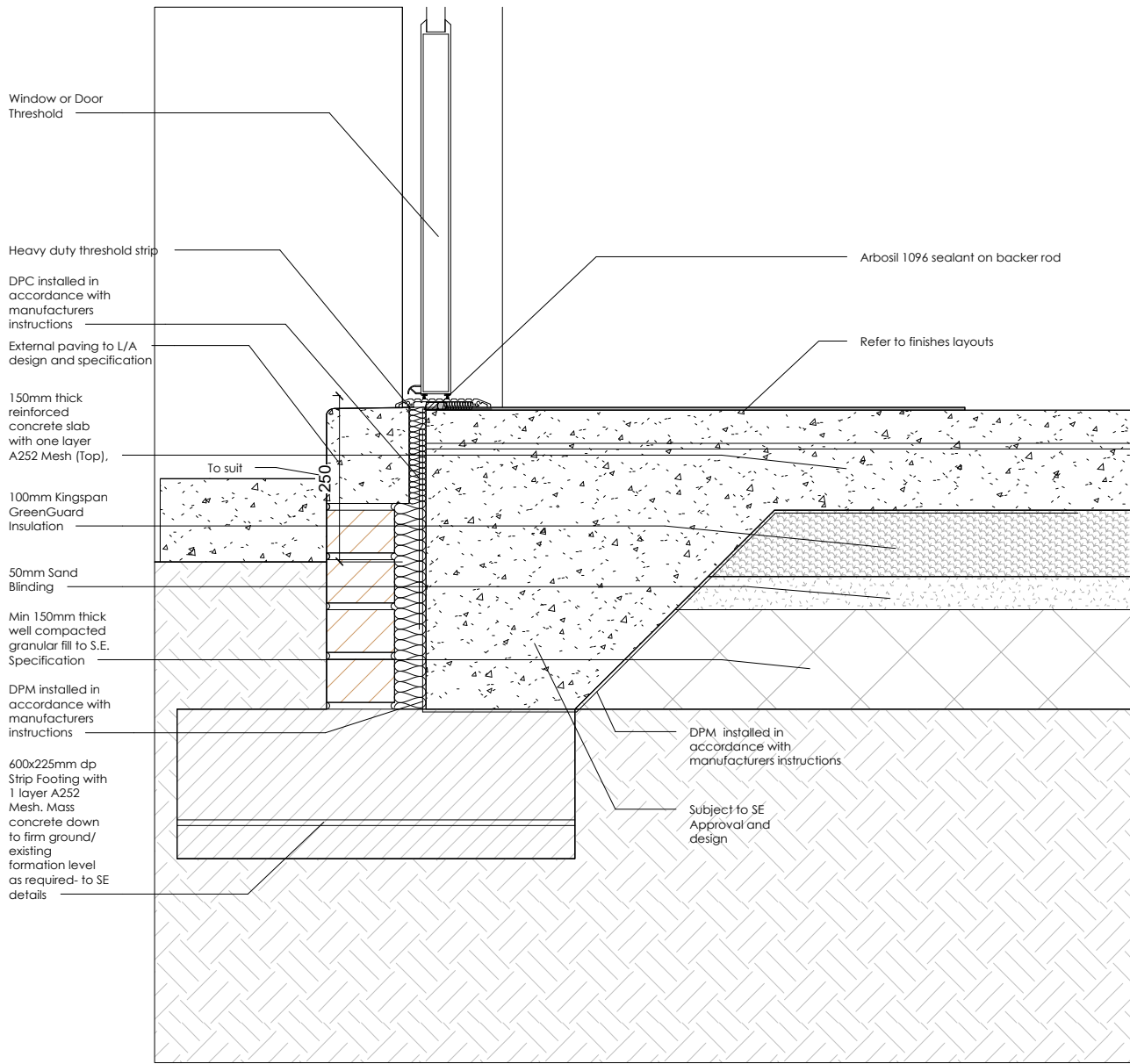
1 Lean-To Foundation and Glazing Junction Detail 1 : 10
