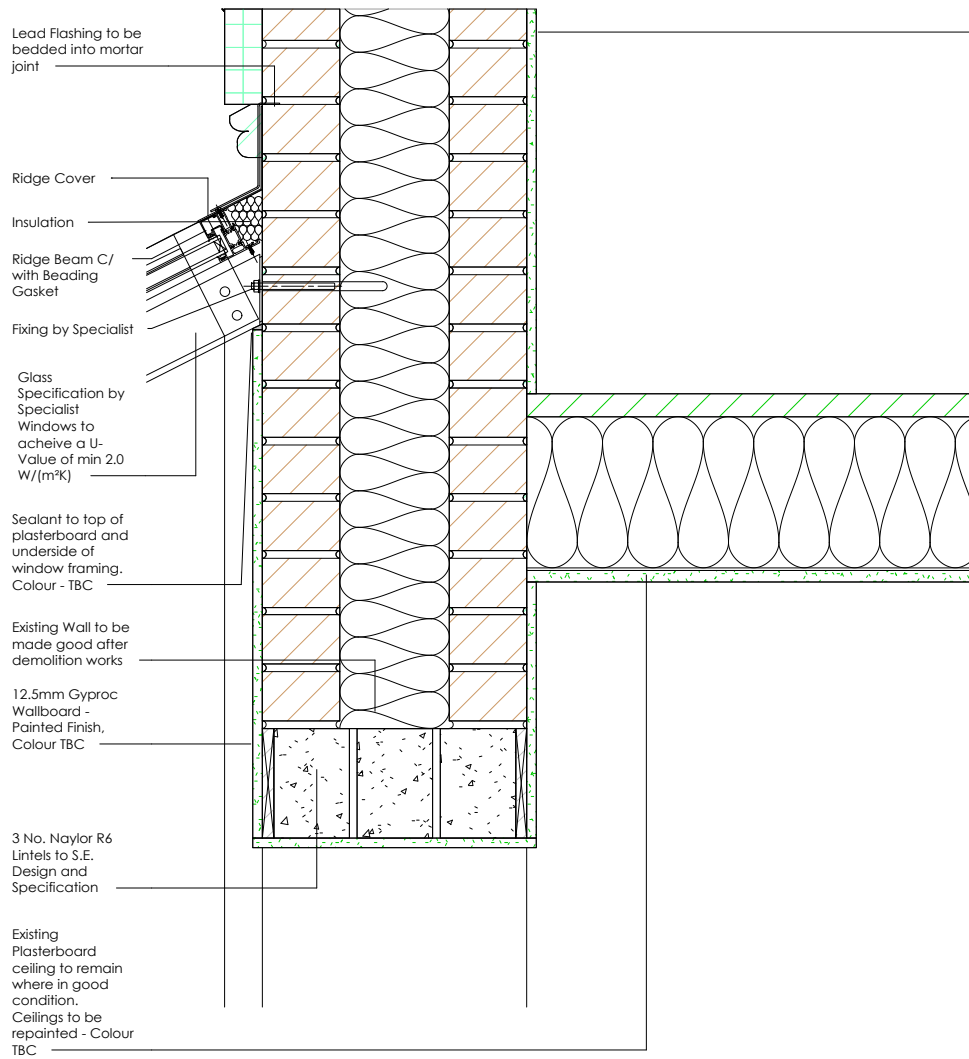
2 Lean-To Connection to Existing Wall Detail 1 : 10
