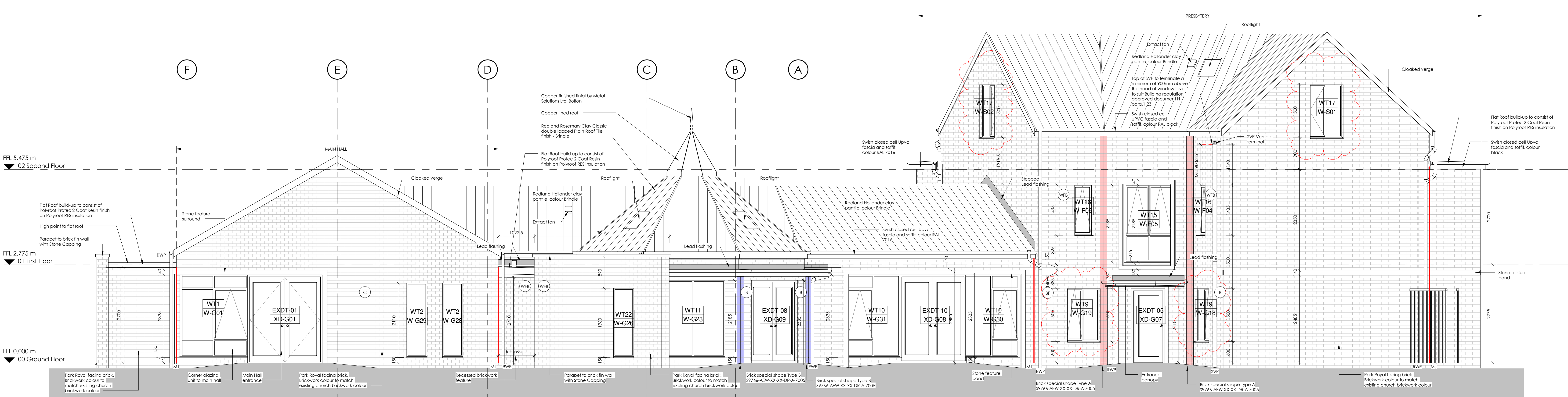
North Facing Elevation Scale @ 1 : 50
