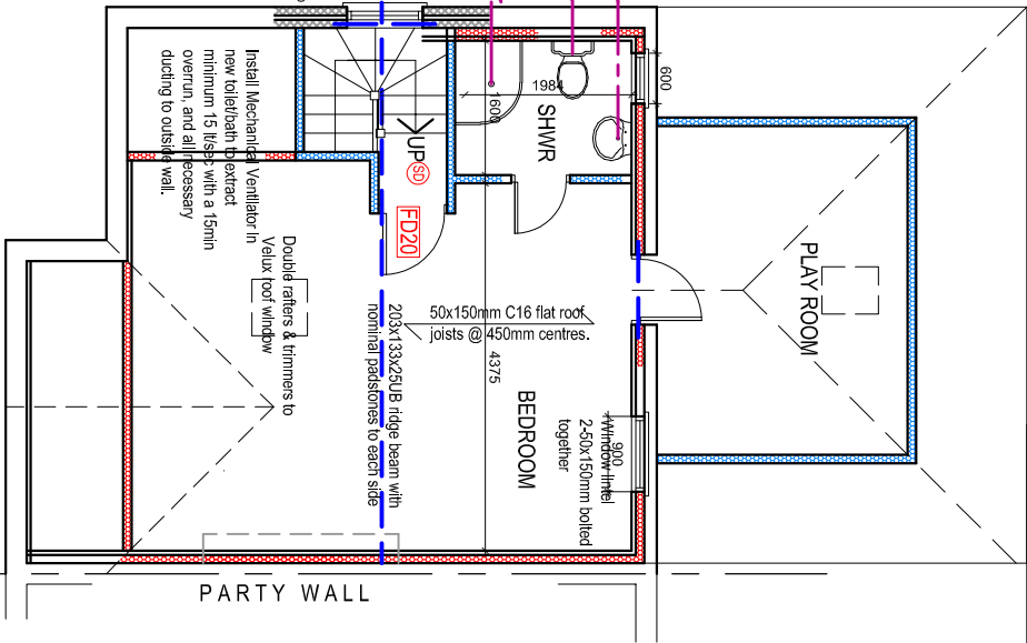
PROPOSED LOFT PLAN
