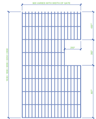
MESH PANEL CUT DETAILS SCALE 1:10
