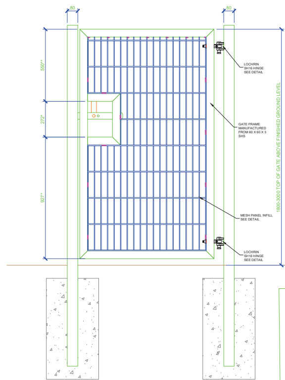
SINGLE LEAF GATE EXTERNAL ELEVATION CENTRE HUNG - OPENING IN / OUT SCALE 1:10
