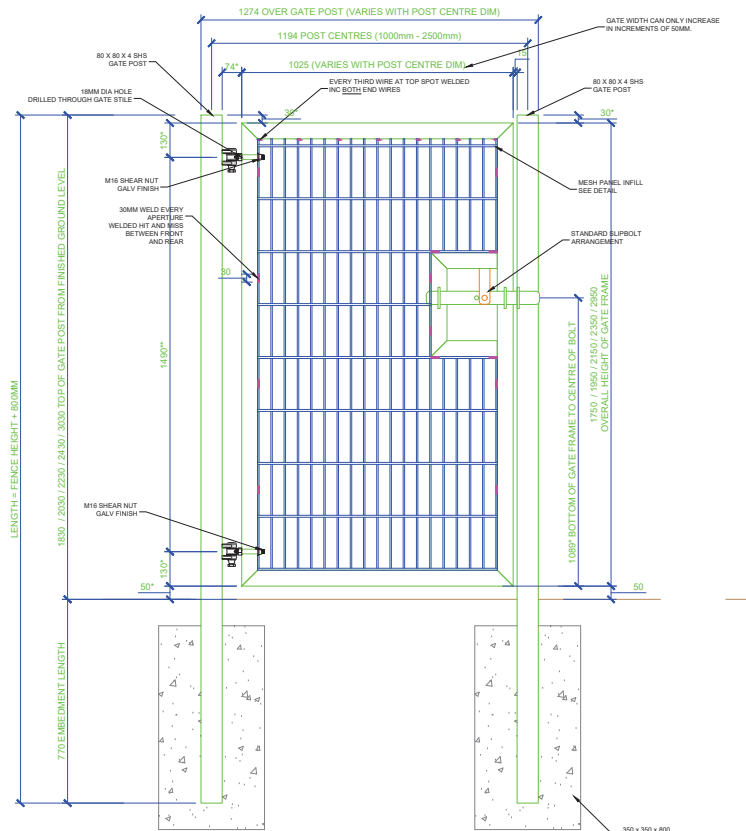
SINGLE LEAF GATE INTERNAL ELEVATION CENTRE HUNG - OPENING IN / OUT SCALE 1:10
