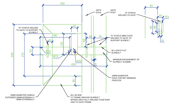
LOCKING ARRANGEMENT SCALE 1:5
