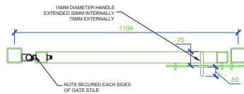
GATE PLANS OPEN &amp; CLOSED
