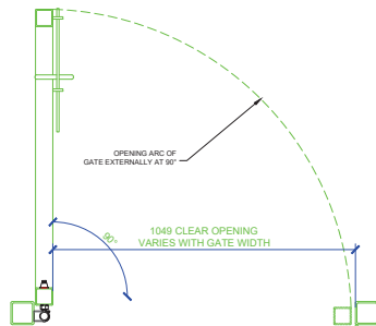
GATE PLANS OPEN &amp; CLOSED
