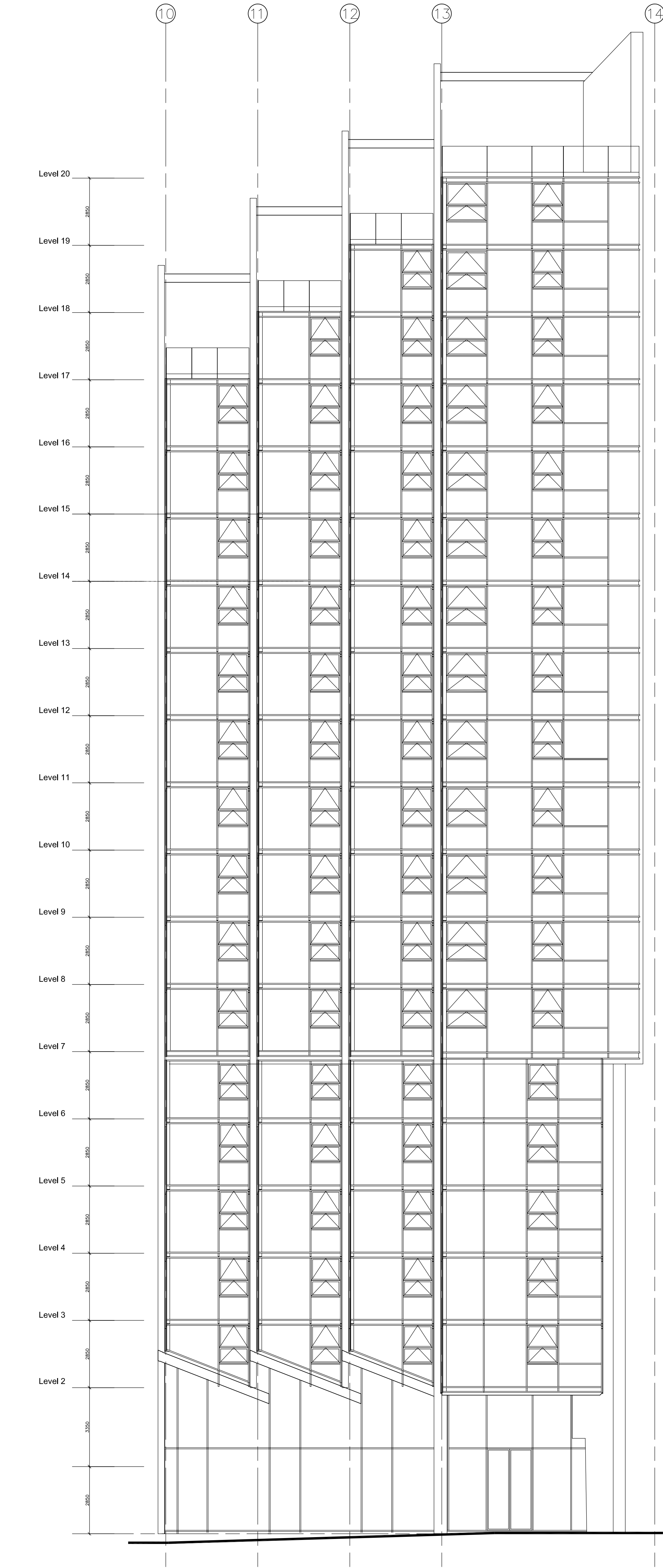
BLOCK B - Elevation D As Proposed
