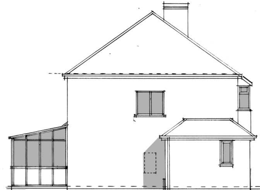
South Elevation
