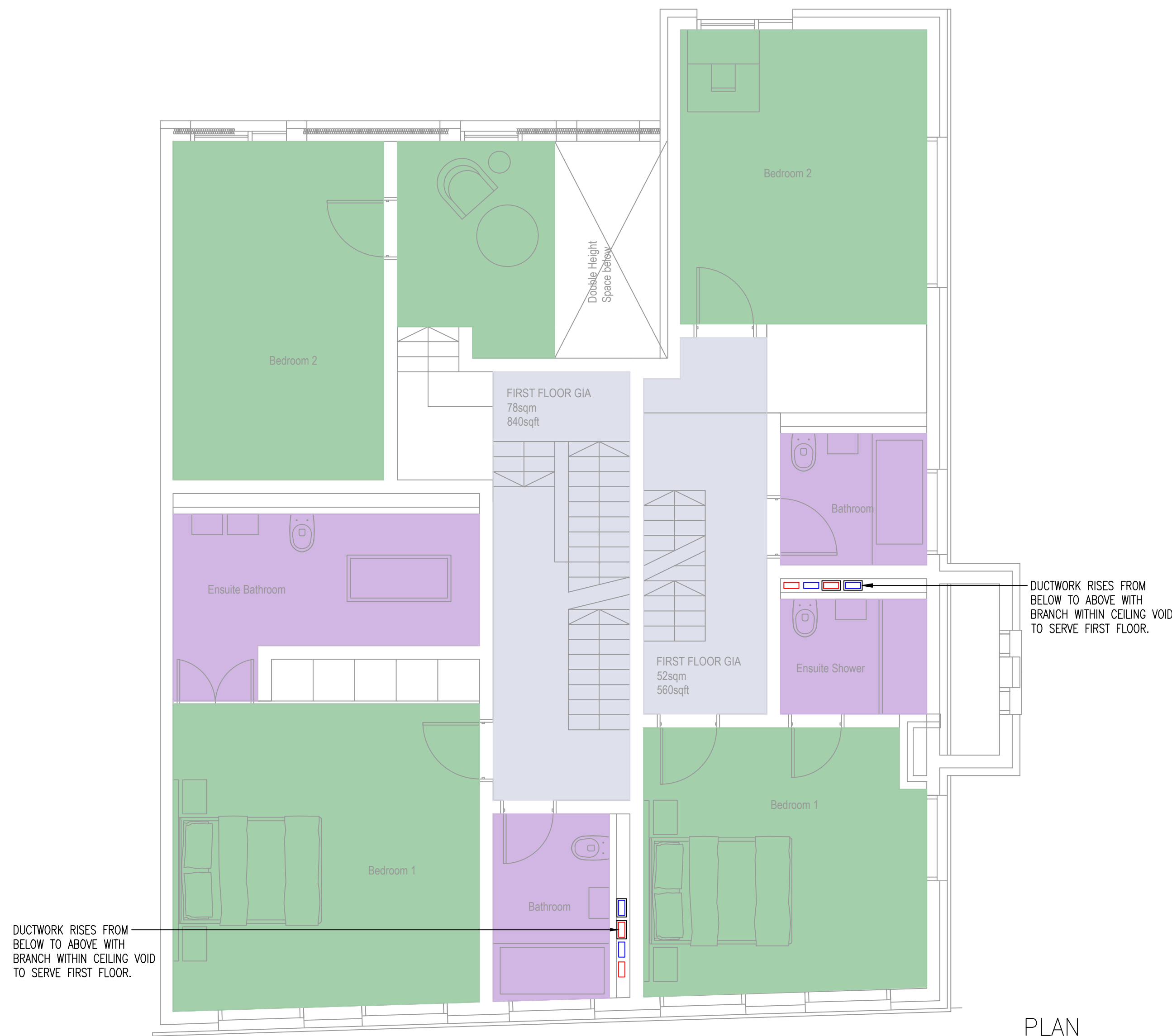
PLAN Proposed First Floor 1:50
