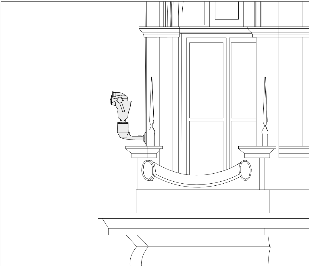
Proposed camera 27 (side view) Esc. 1:25
