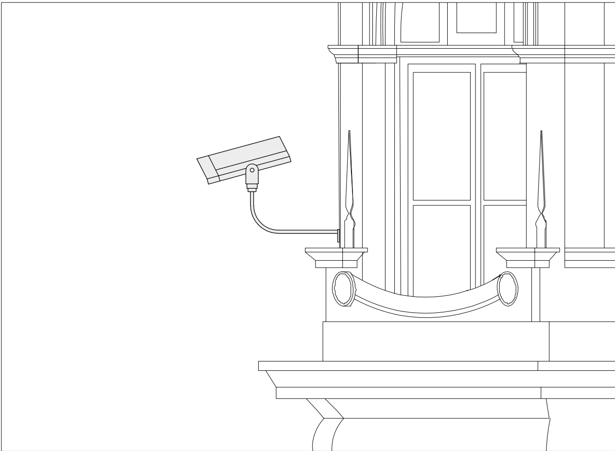
Existing camera 27 to be replaced (side view) Esc. 1:25
