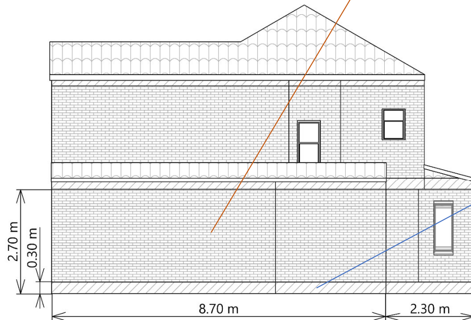
Proposed Side Elevations
