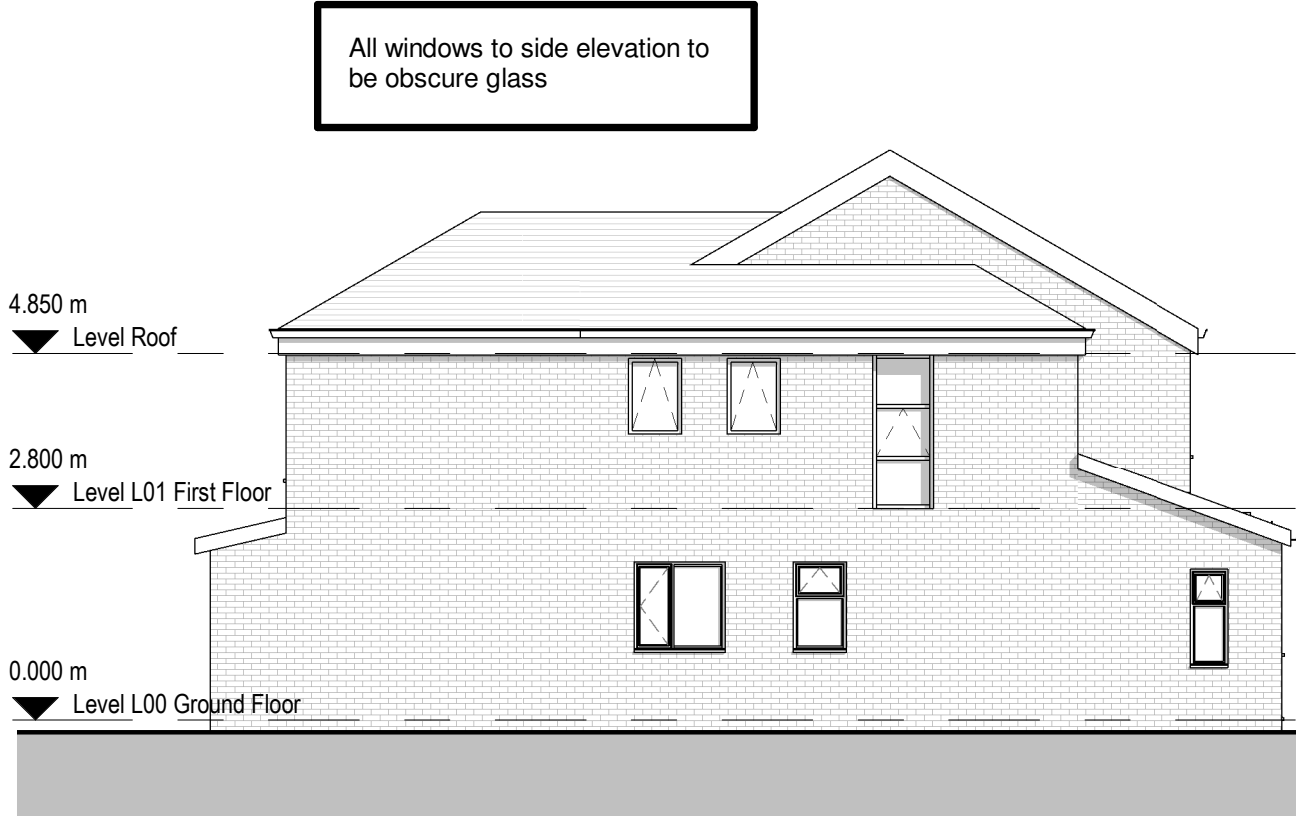
2 Proposed East Elevation 1 : 100
