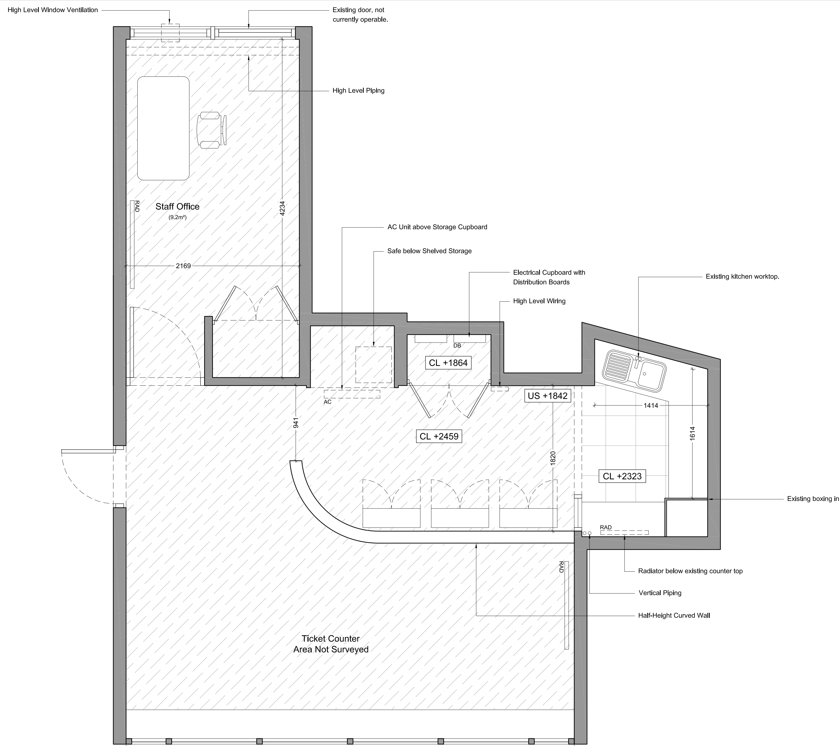
Area A - Existing Ticket Office GA Plan Scale 1 : 25
