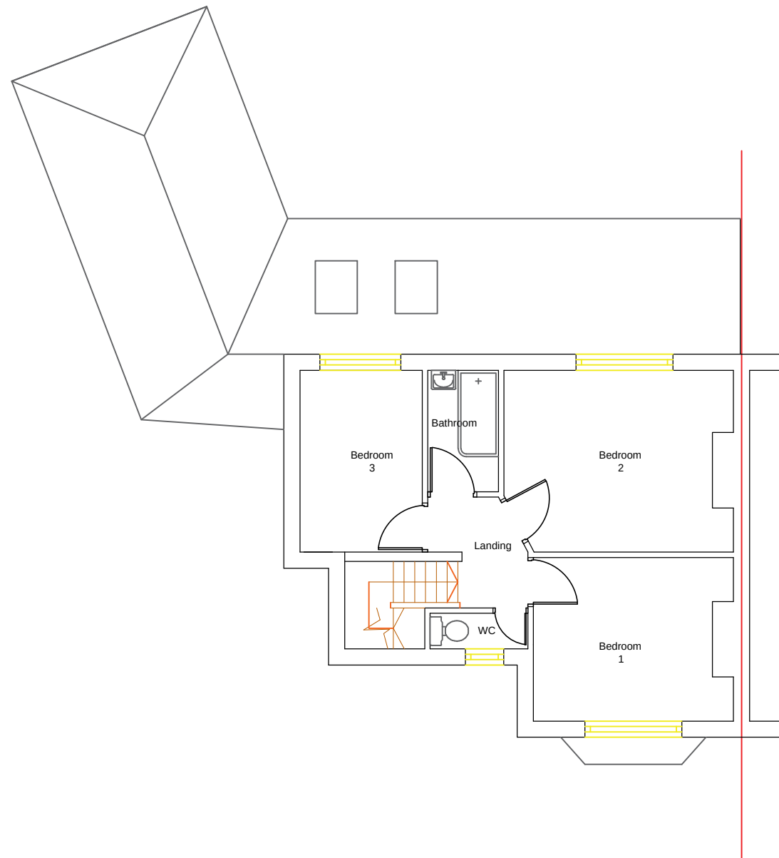
EXISTING 1ST FLOOR
