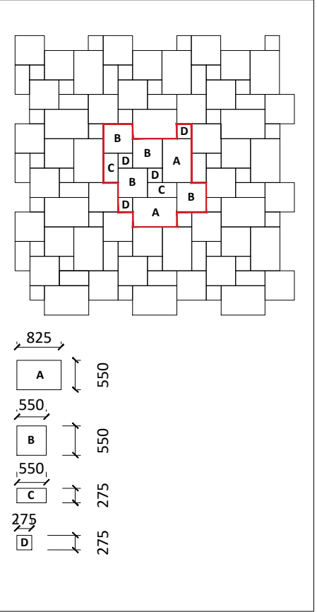
Proposed Opus Paving Detail 1:100@A3
