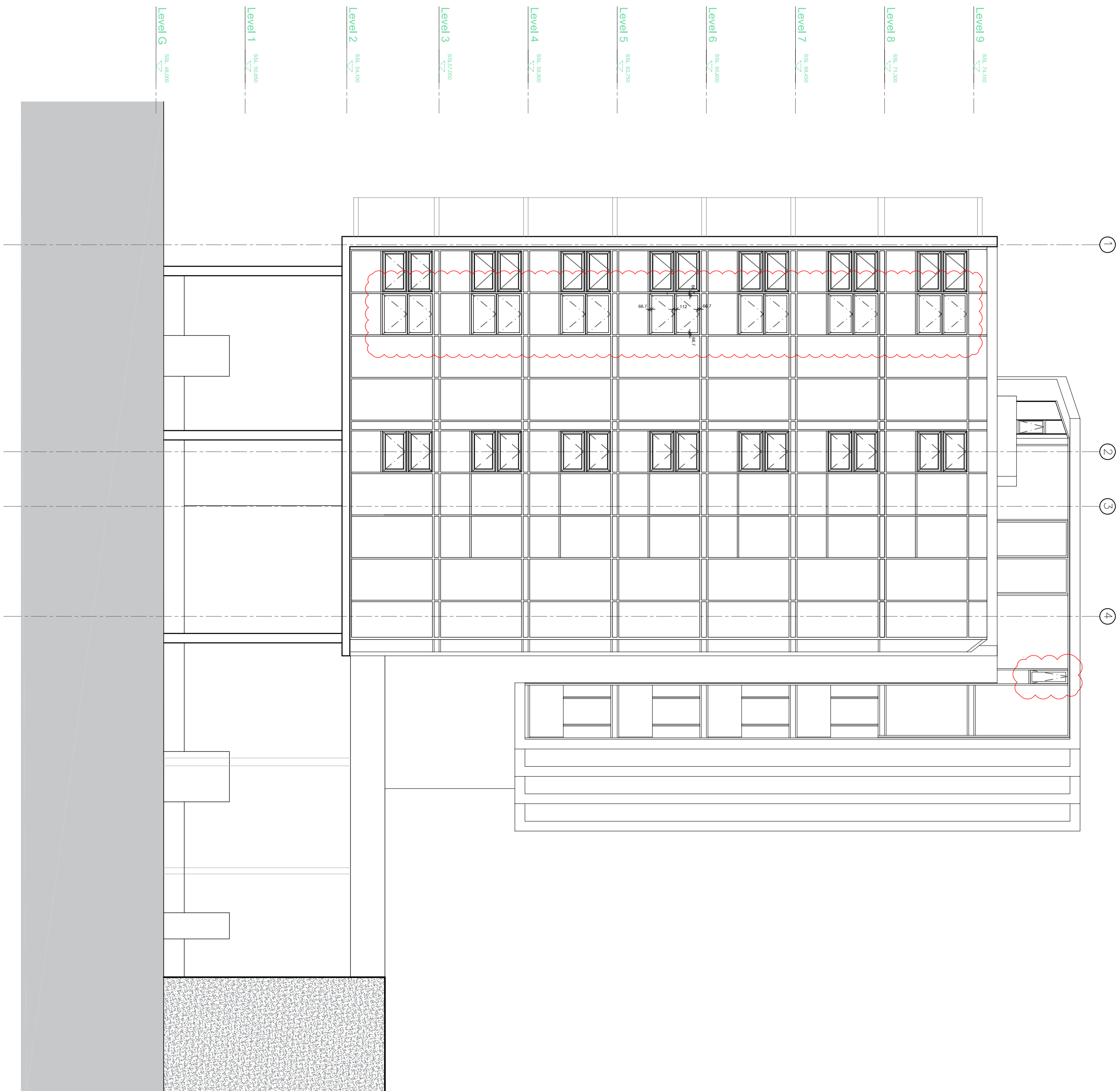
BLOCK A - Elevation B as proposed
