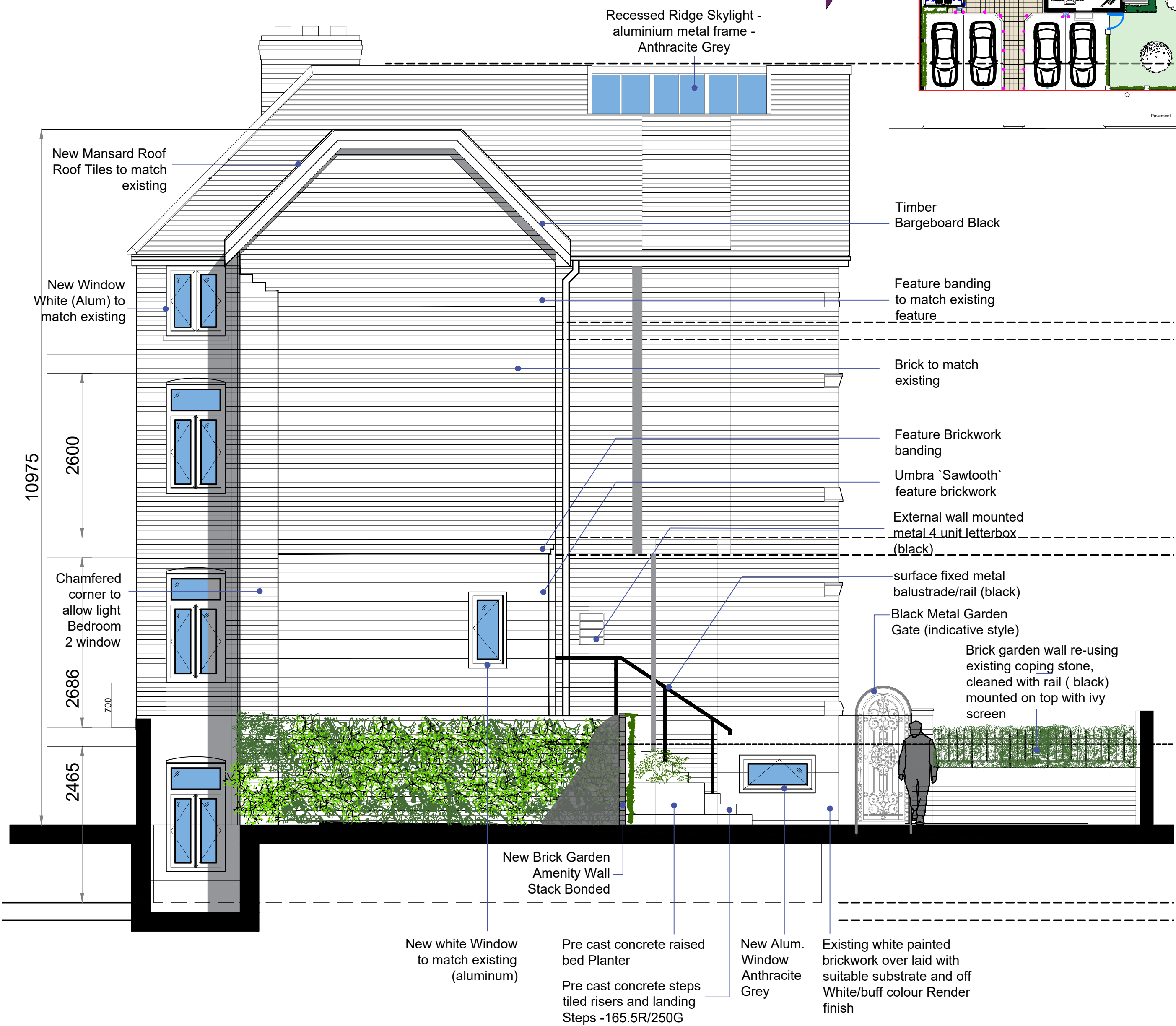
Proposed Side Elevation A 1:50
