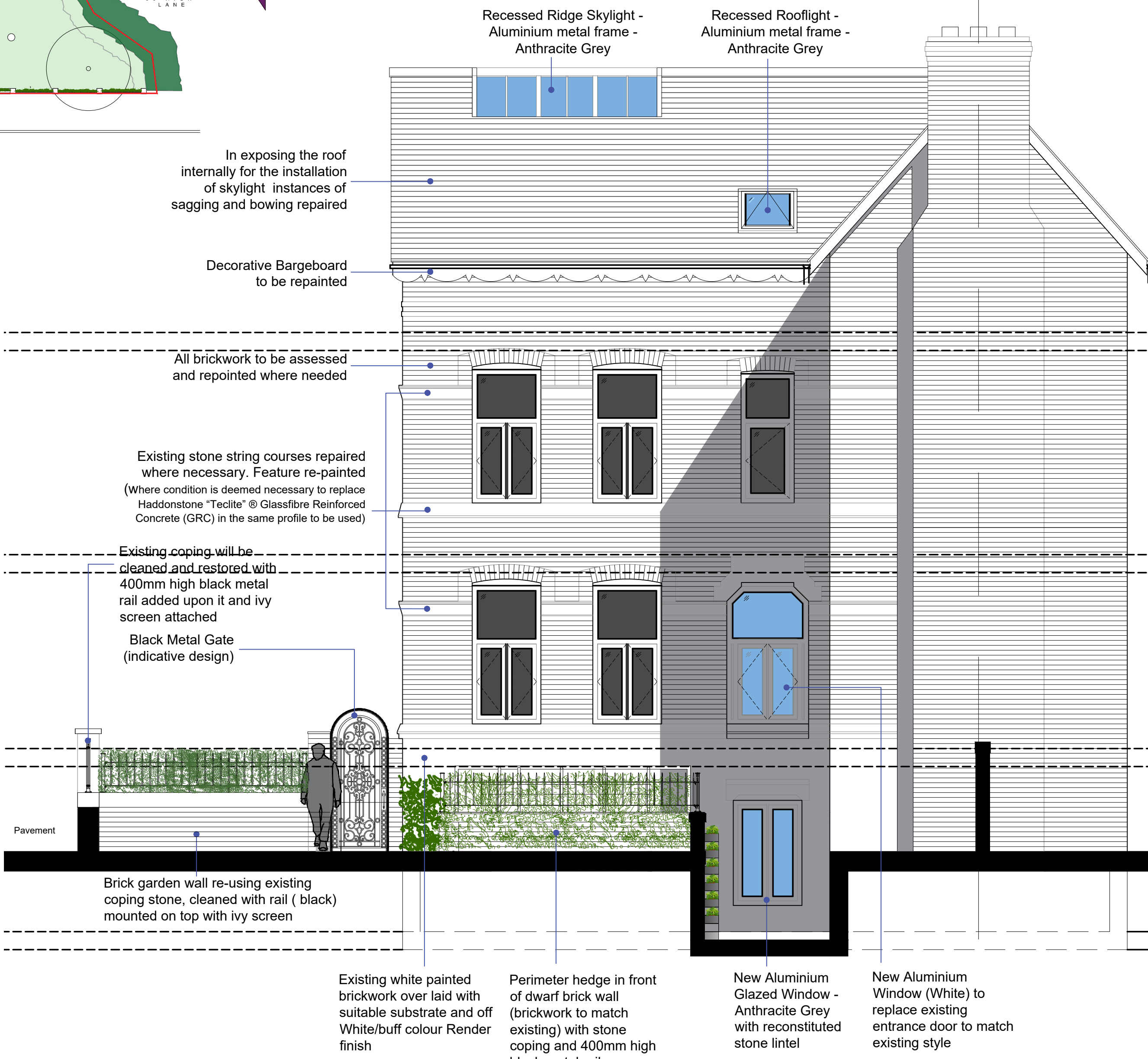
Proposed Side Elevation B 1:100
