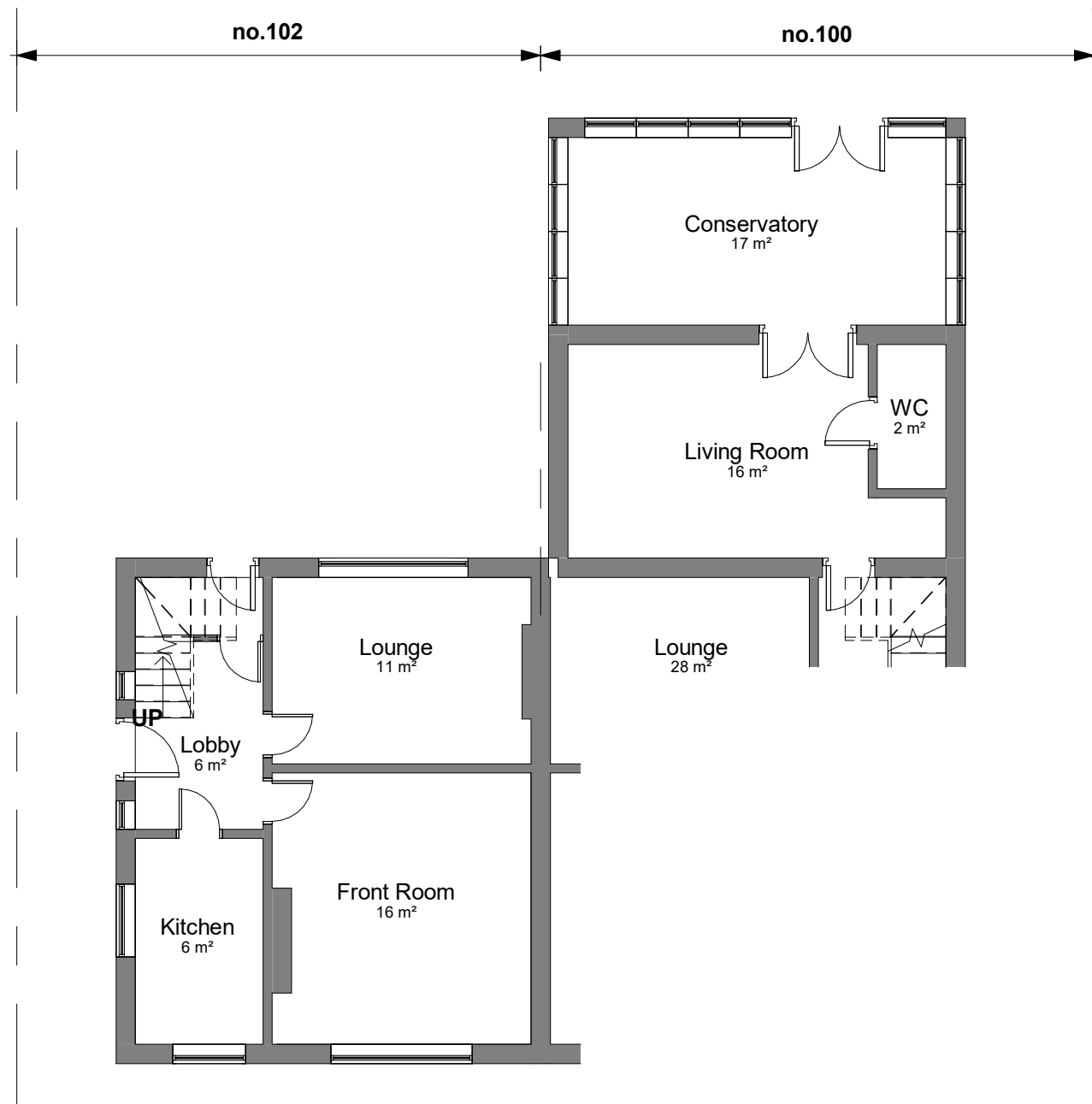
00-E-Ground Floor 1 : 100
