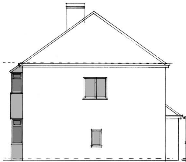
North Elevation
