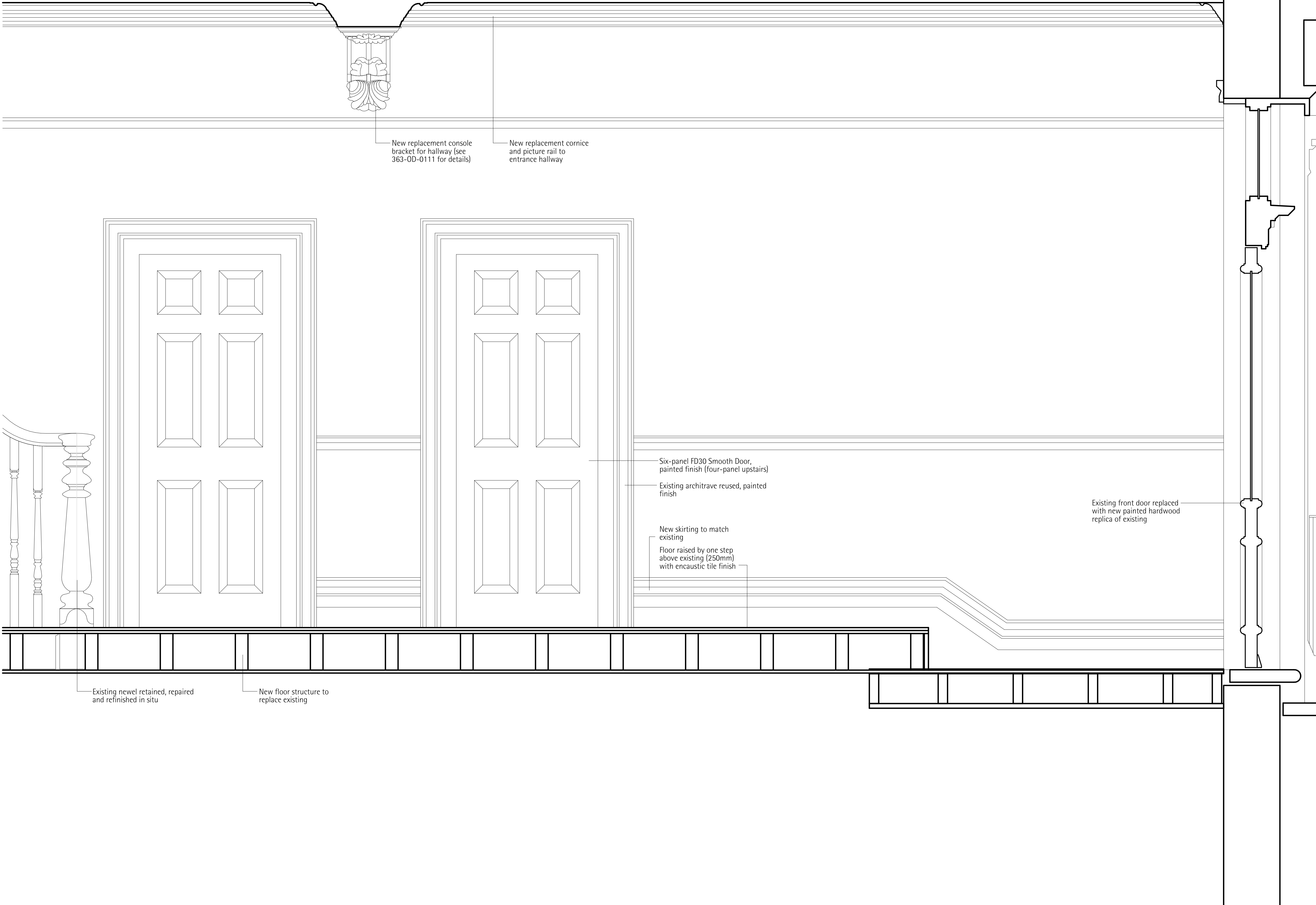
Hallway Section 1:10
