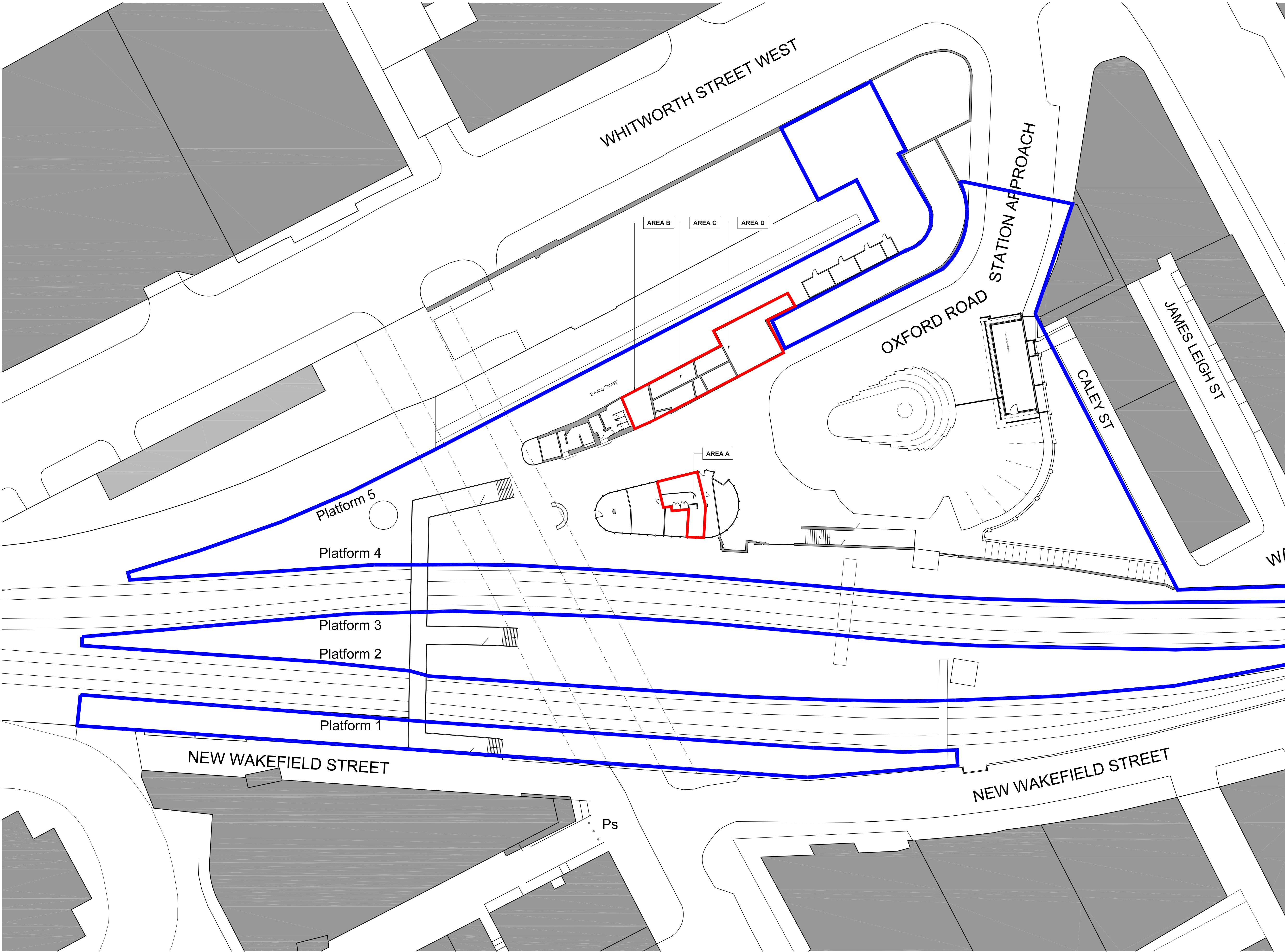
Existing Site Location Plan Scale 1 : 250
