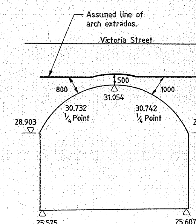
SECTION THROUGH ARCH 1A
