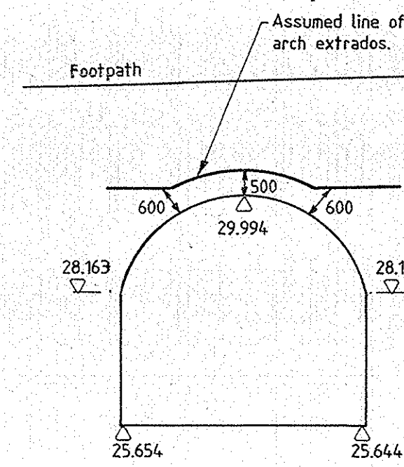
SECTION THROUGH ARCH 12
