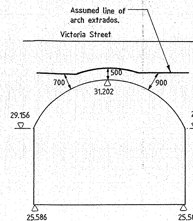
SECTION THROUGH ARCH 3A
