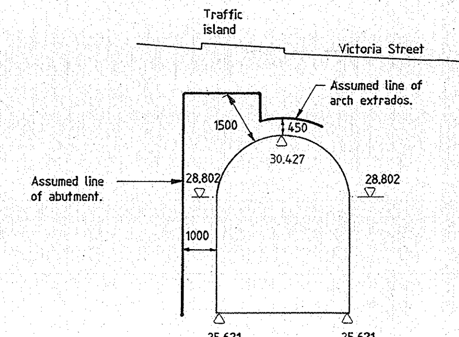
SECTION THROUGH ARCH A
