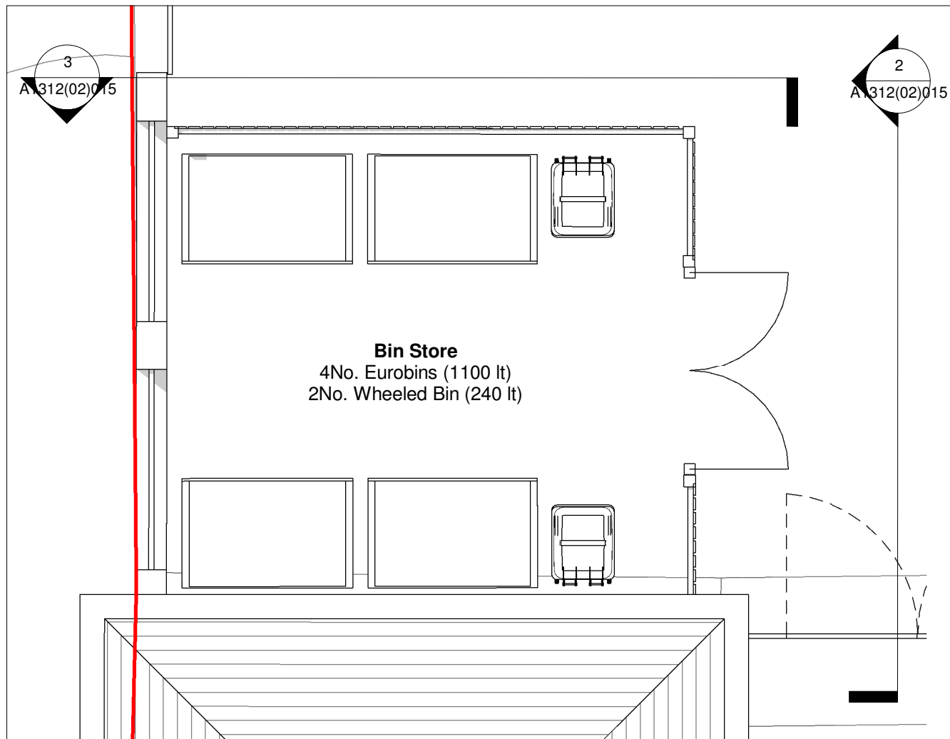
1 Proposed Bin Store Plan 1 : 50
