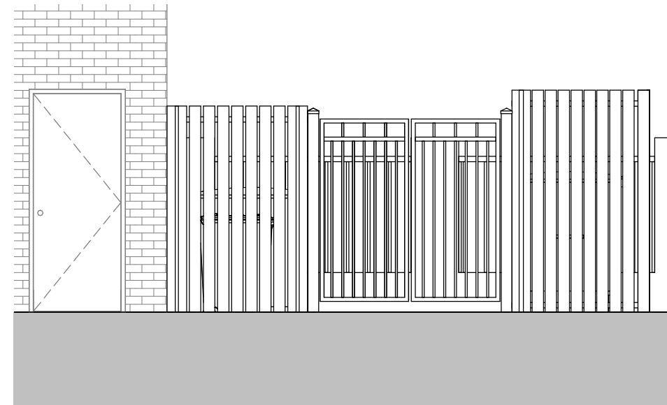
2 Bin - Front Elevation 1 : 50
