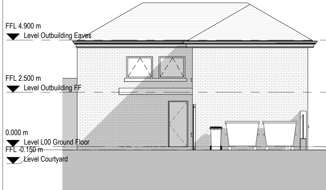
1 Outbuilding North 1 : 100
