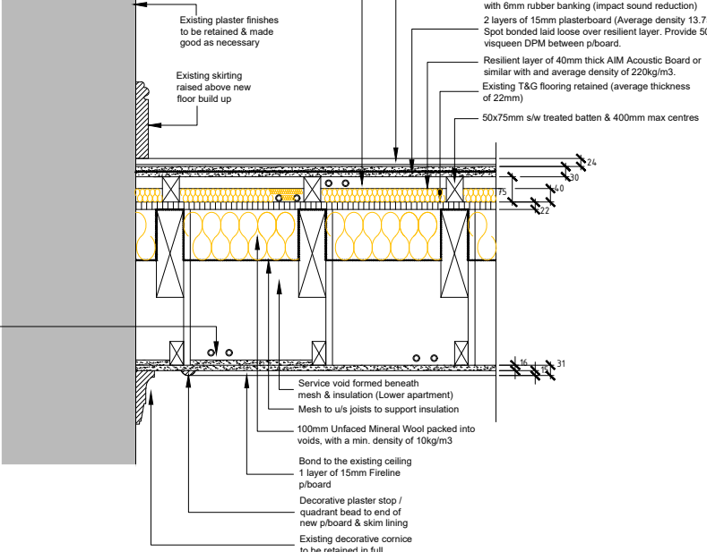
Proposed Section
