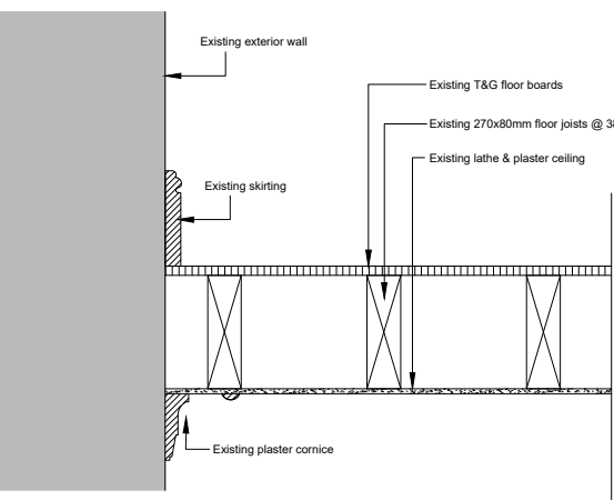
Existing Section
