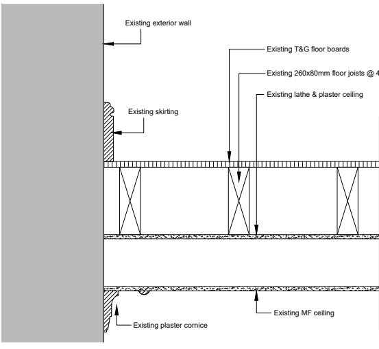
Existing Section
