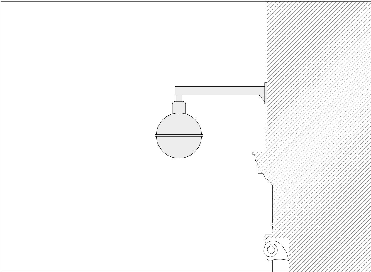
Existing camera 26 to be replaced (cross section) Esc. 1:25
