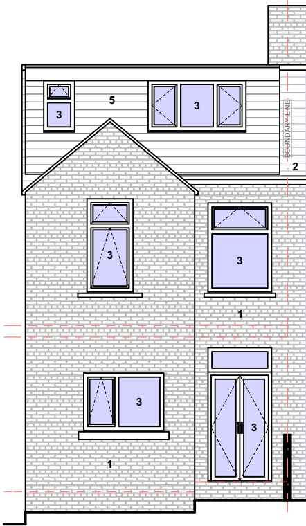
EXISTING GA REAR ELEVATION @1:100
