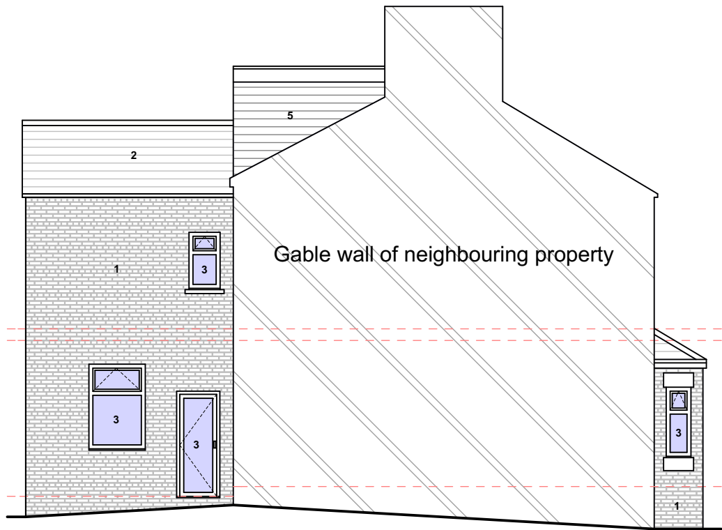
EXISTING GA SIDE ELEVATION 2 @1:100
