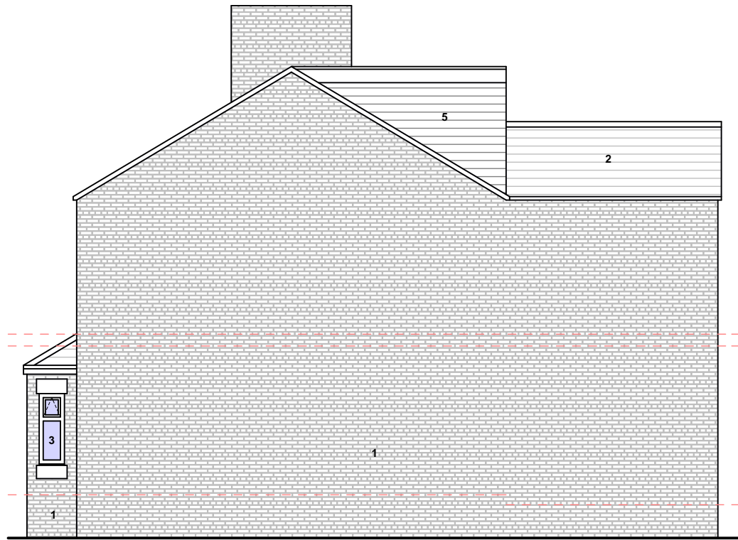
EXISTING GA SIDE ELEVATION 1 @1:100
