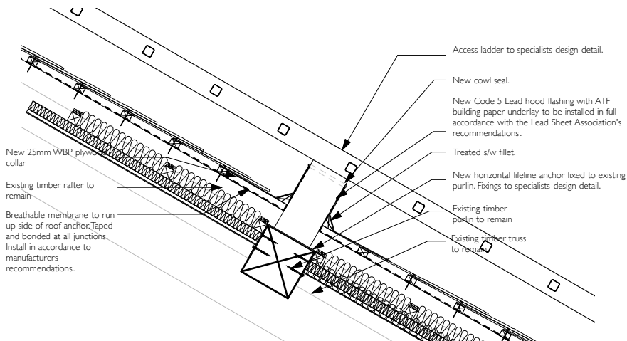
Deatil 3 Ladder ancor detail
