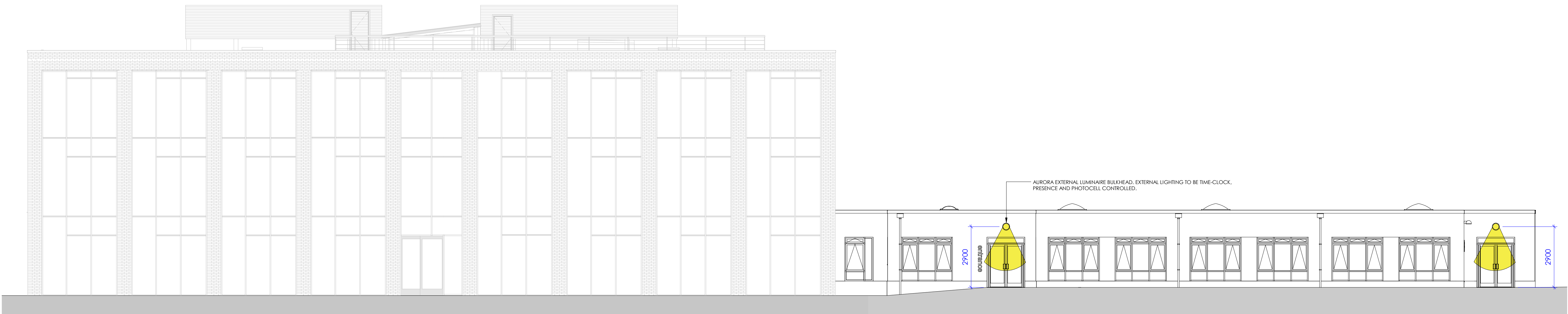
South West Ext. Lighting Elevation 1 : 100
