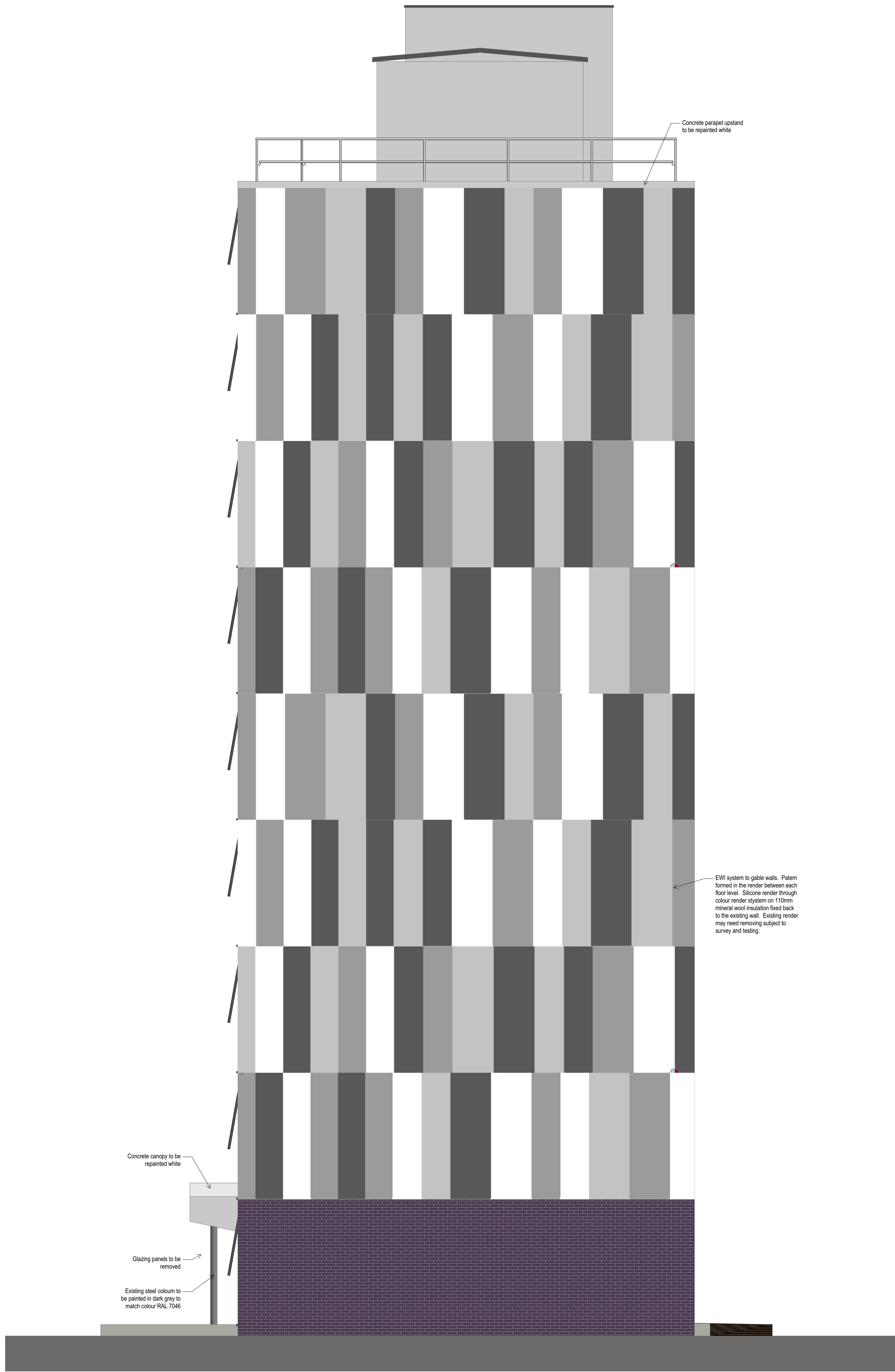
1 Gable Elevations 1:50
