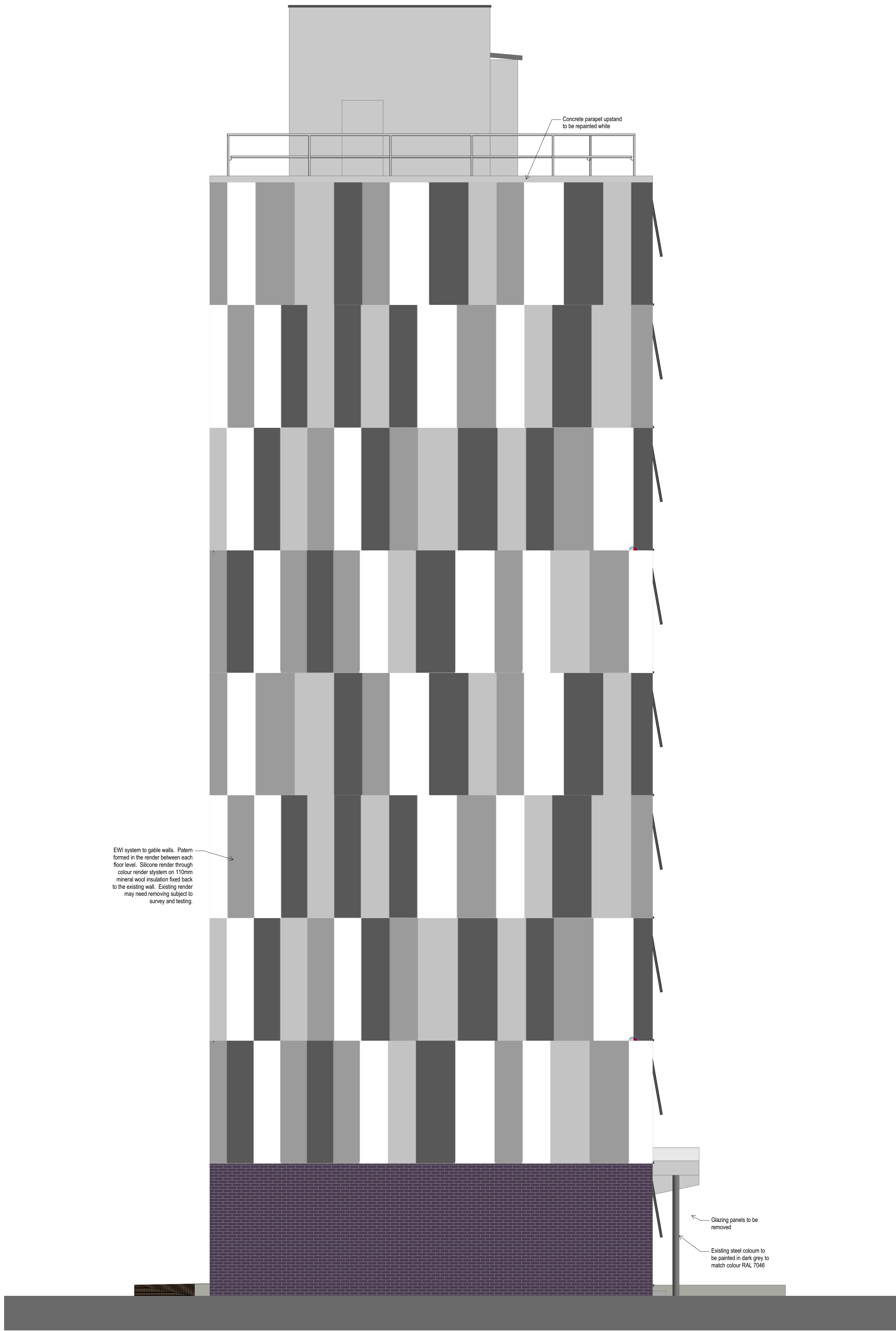
2 Gable Elevations 1:50
