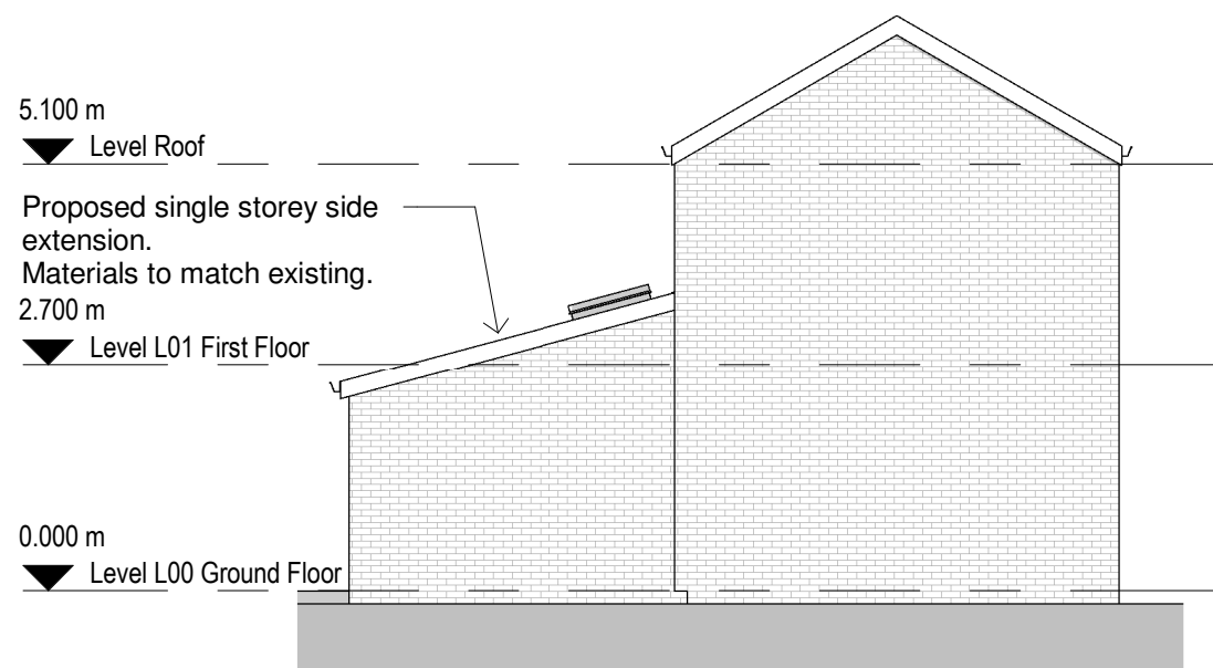
3 Proposed South Elevation 1 : 100
