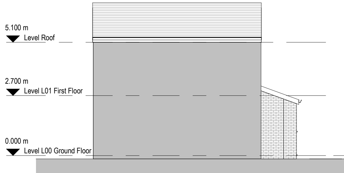
2 Proposed East Elevation 1 : 100
