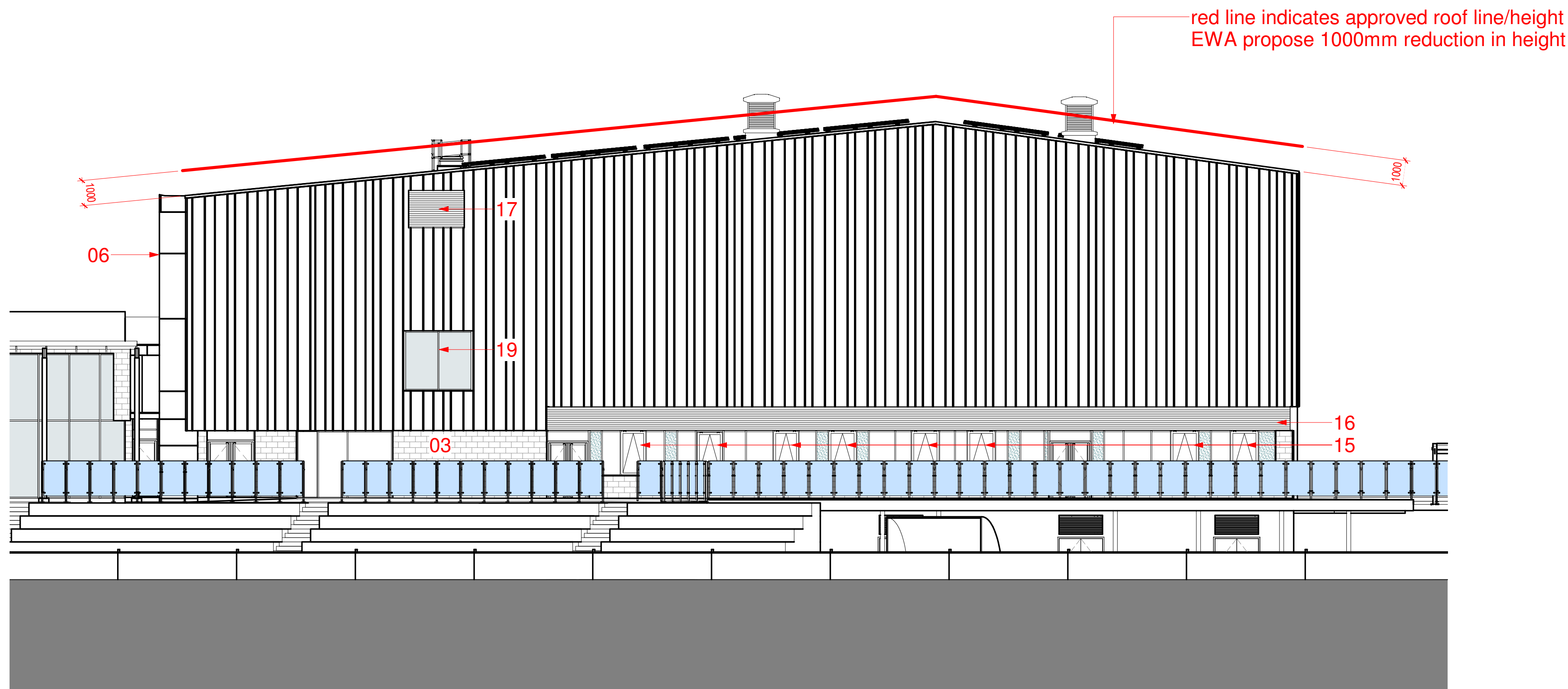
4 SITE-West Elevation - SH & WS 1:125
