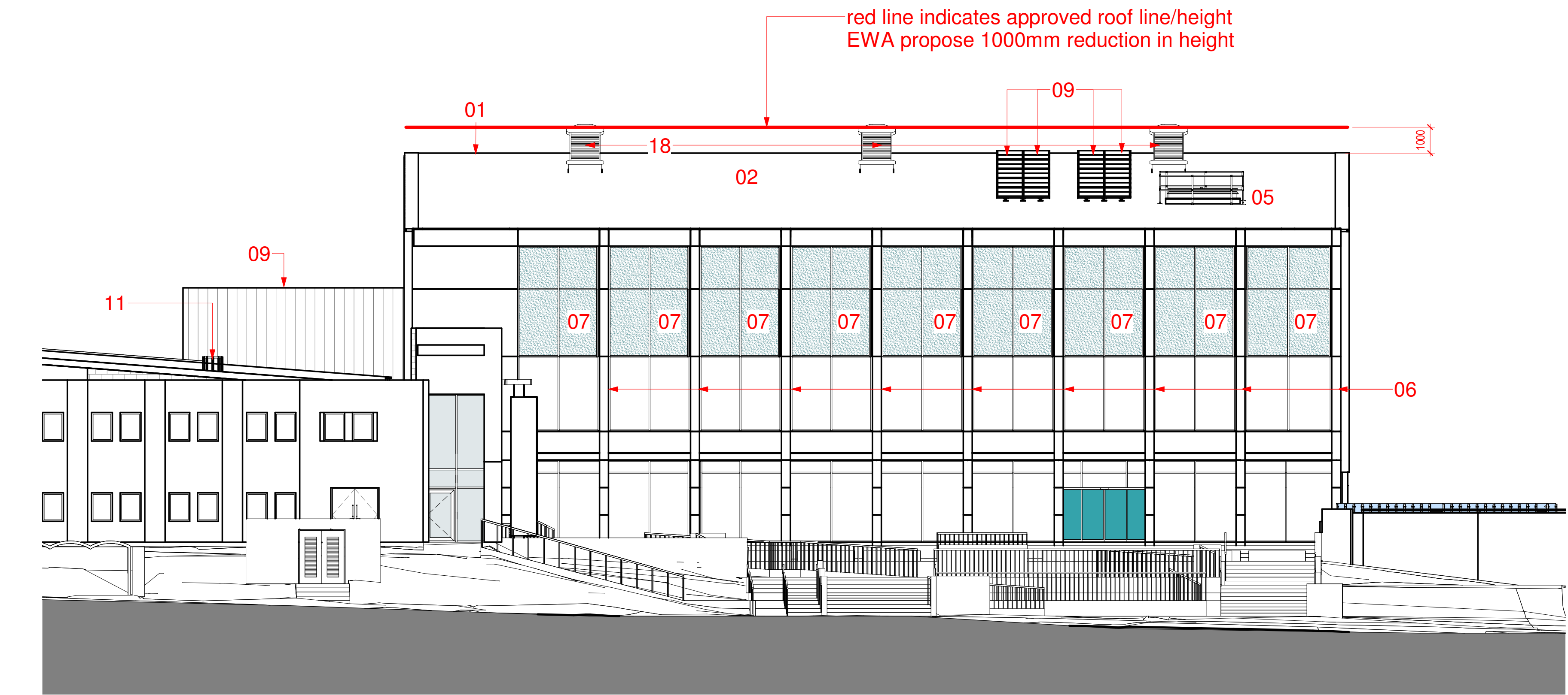
2 SITE-North Elevation - SH & WS 1:125
