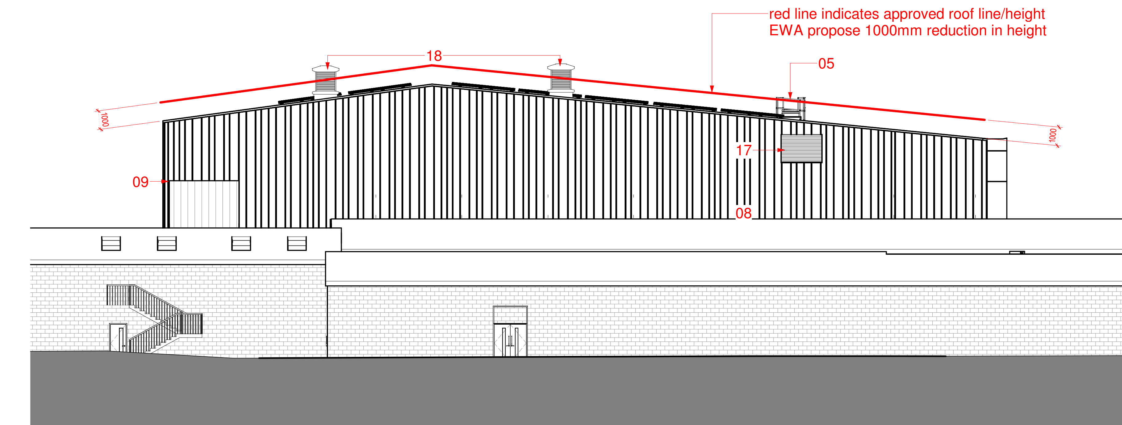
1 SITE-East Elevation - SH & WS 1:125
