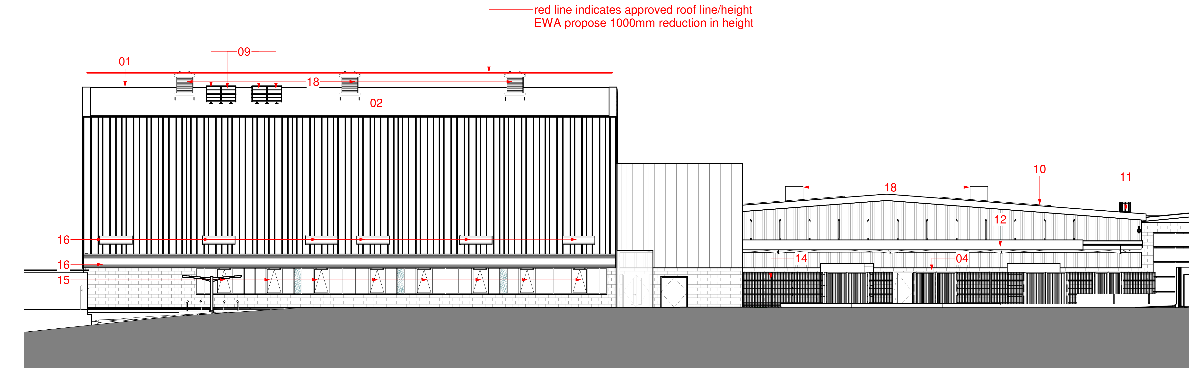
3 SITE-South Elevation - SH & WS 1:125
