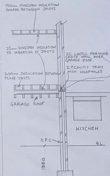
SECTION B:B
