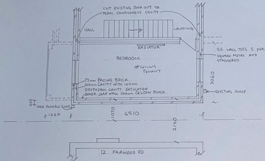
PROPOSED 1 st FLOOR PLAN SCALE 1:50
