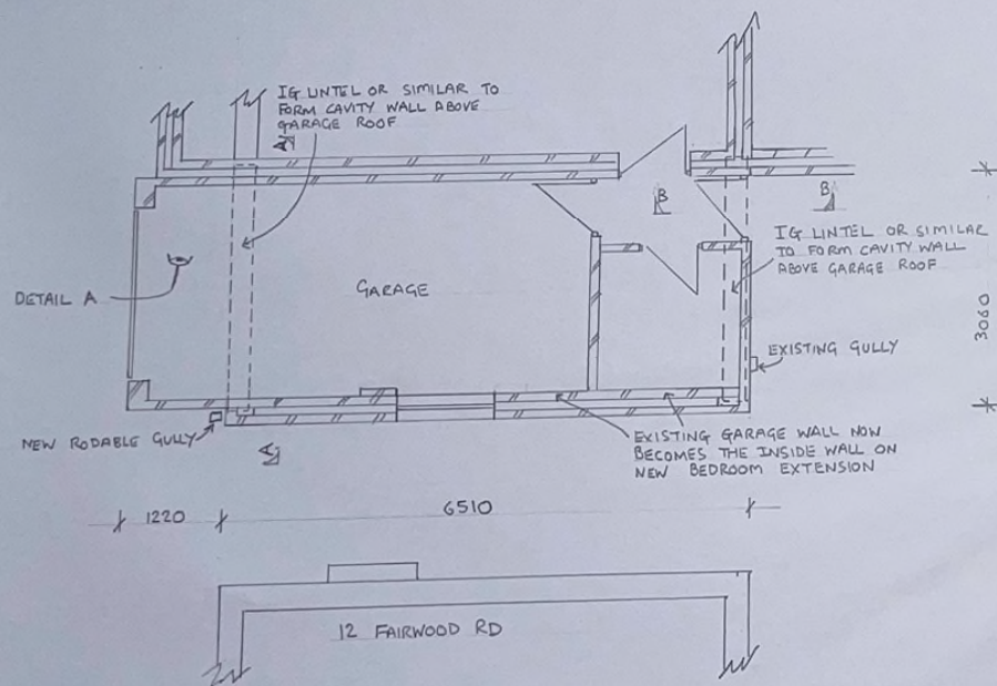
PROPOSED GROUND FLOOR PLAN SCALE 1:50
