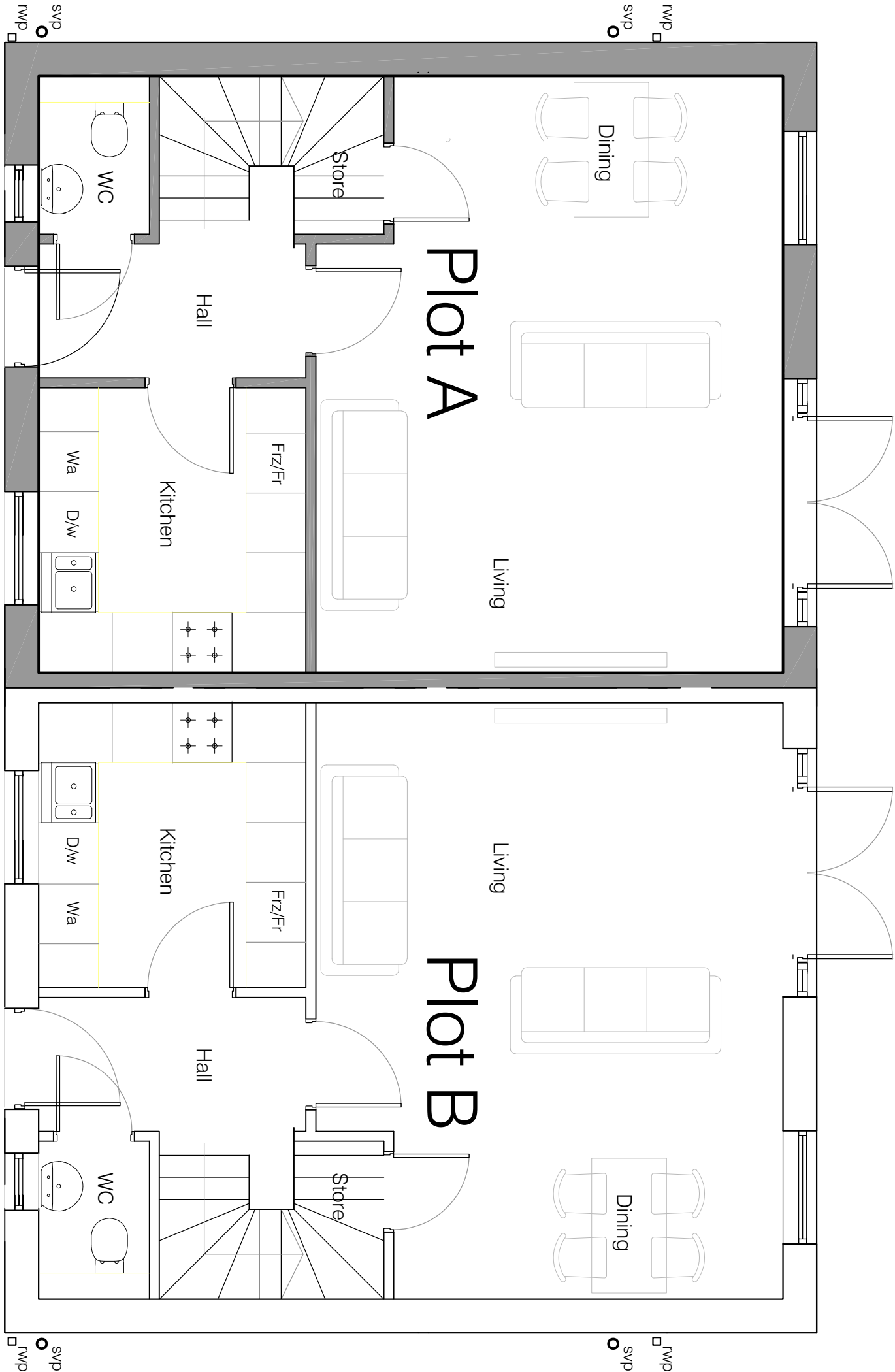
Ground Floor 44.5m2 G.I.A (478 sq ft)
