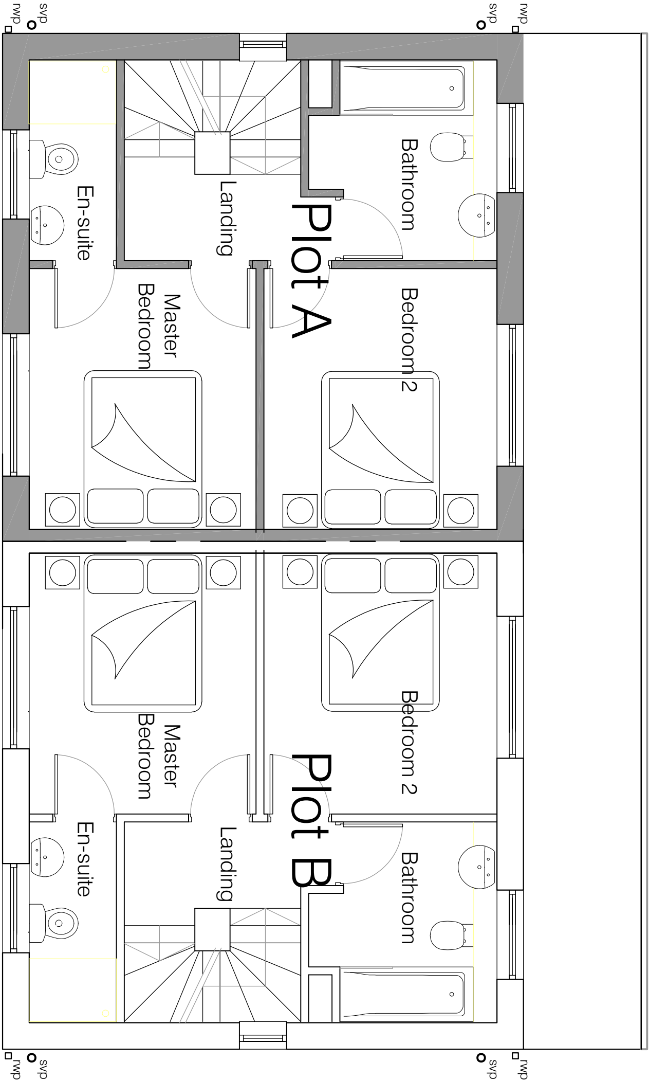
First Floor 35.8m2 G.I.A (385 sq ft)
