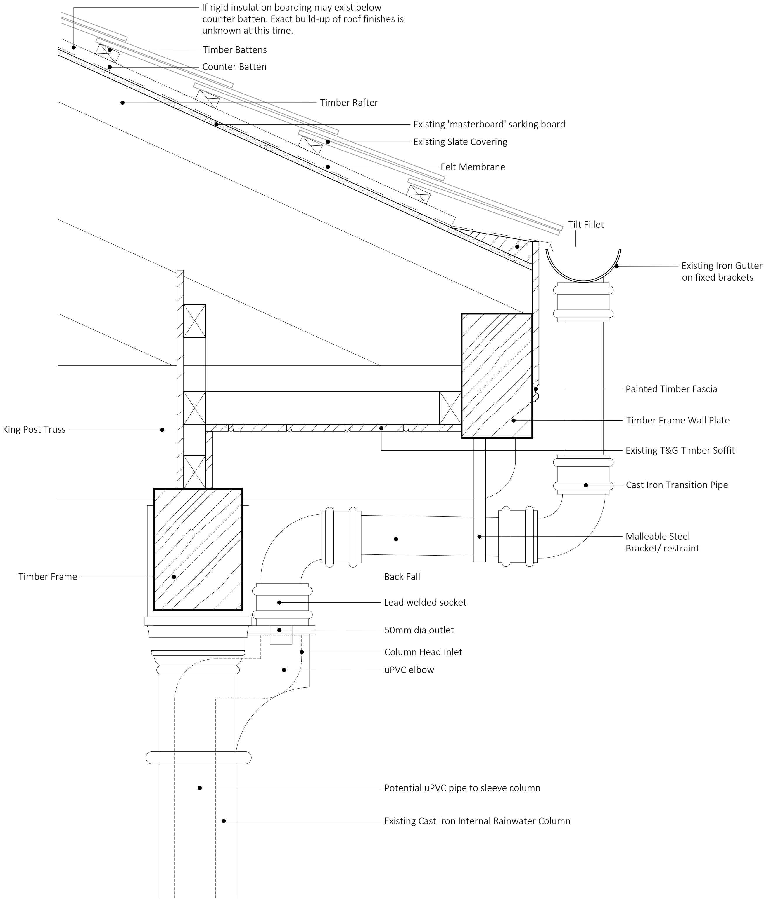
Existing Detail A2 1:5
