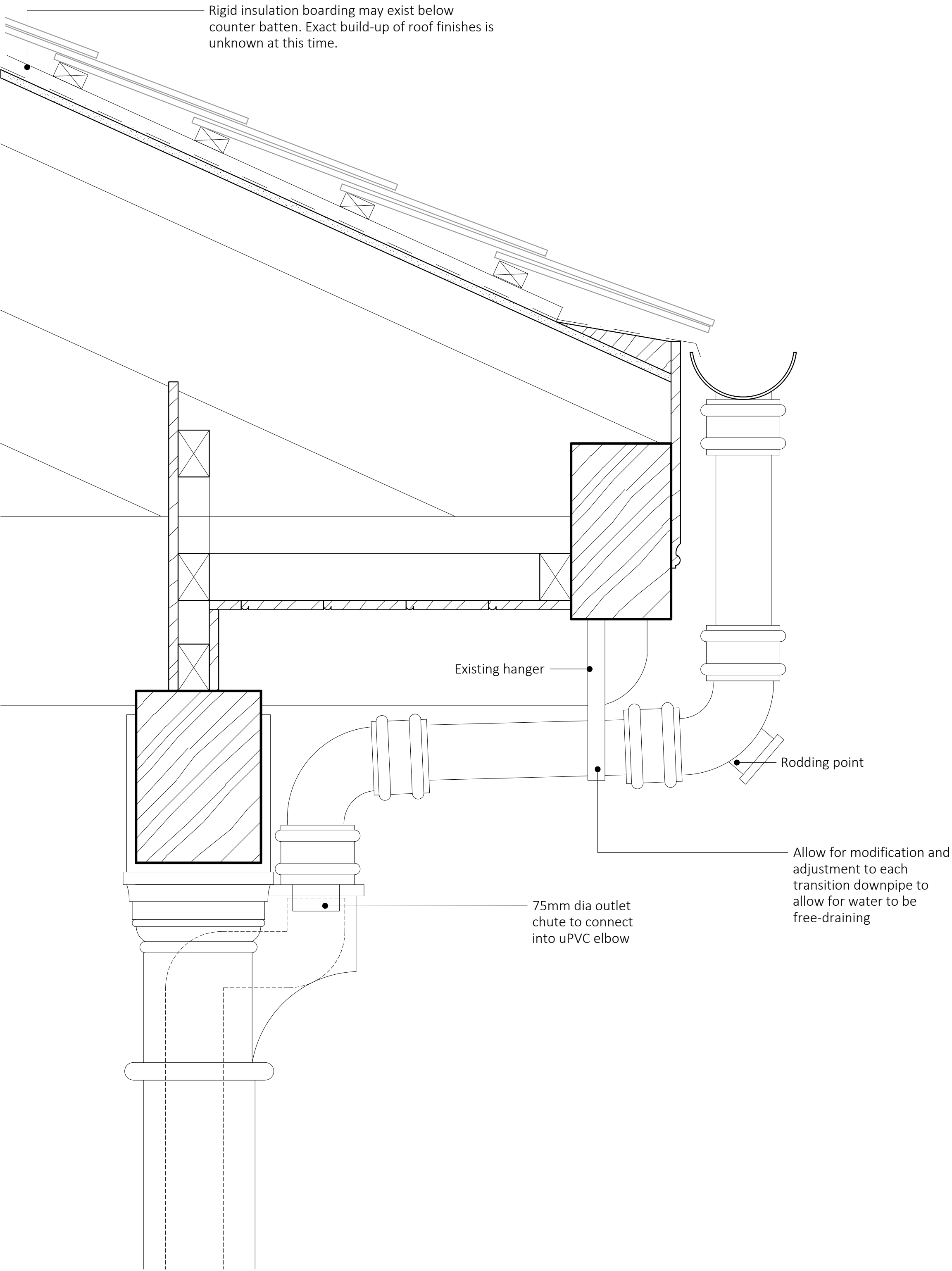
Proposed Detail A2 1:5
