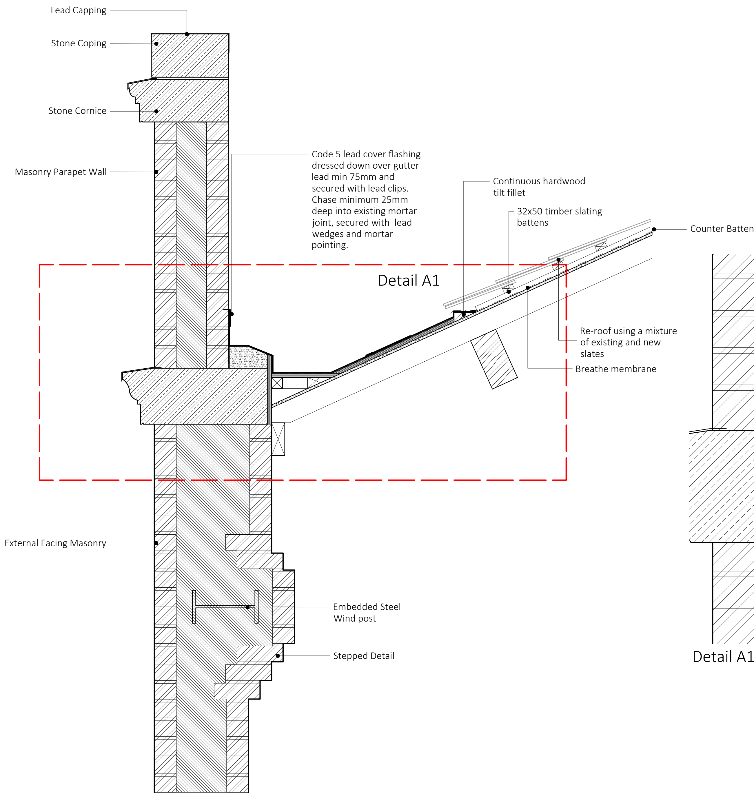
Proposed Parapet Detailed Section A 1:10
