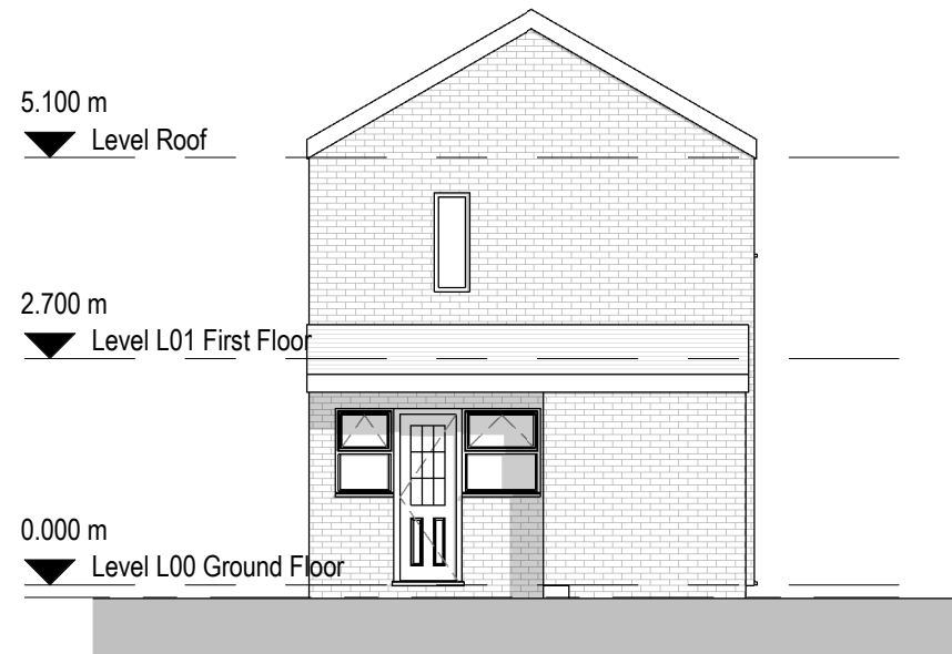
1 Existing North Elevation 1 : 100
