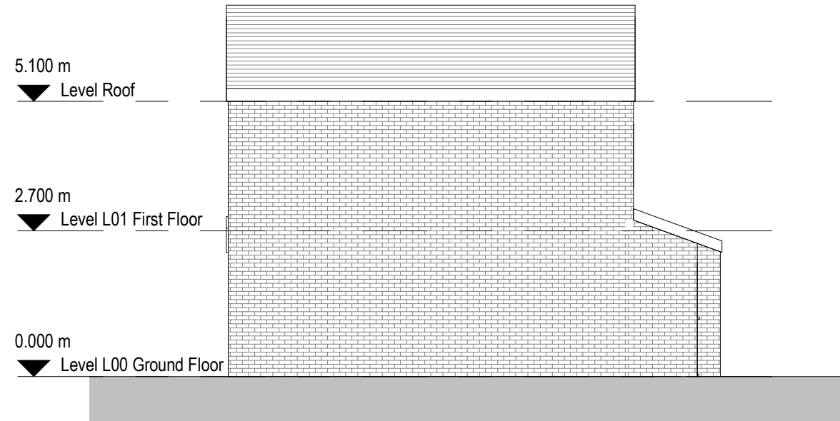
2 Existing East Elevation 1 : 100
