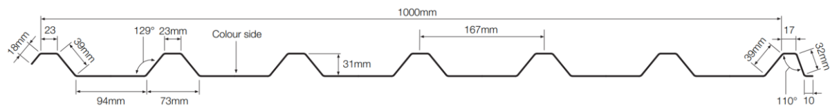
Euroclad 32/1000 R - WALL PROFILE outer sheet, colour Goosewing Grey
