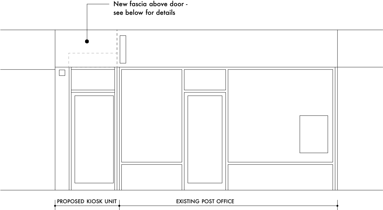
PROPOSED ELEVATION
