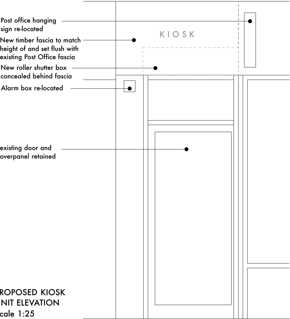
PROPOSED ELEVATION
