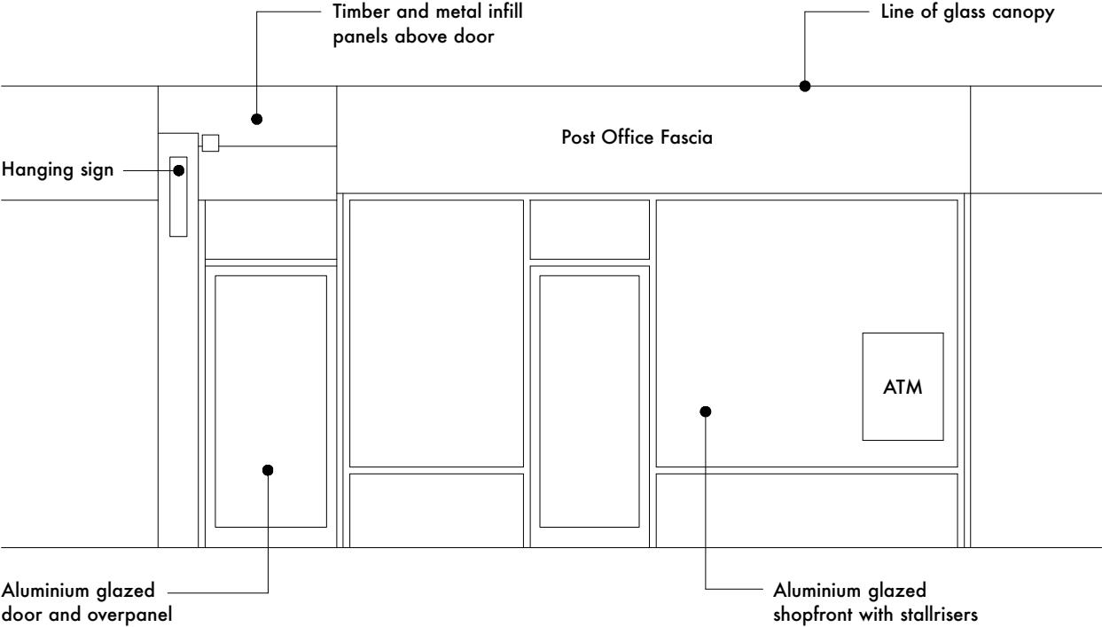
EXISTING ELEVATION
