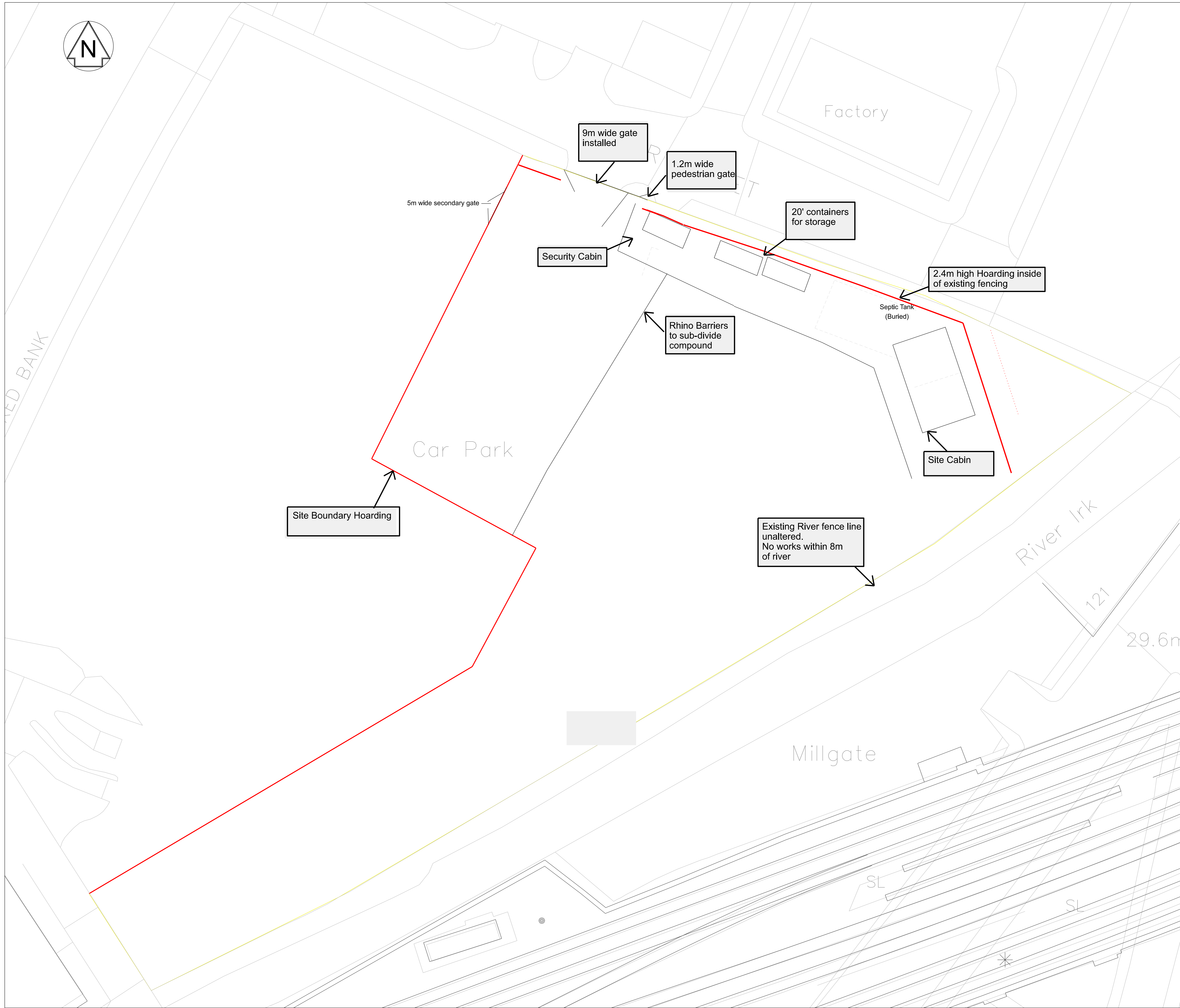
Plan Scale 1:250
