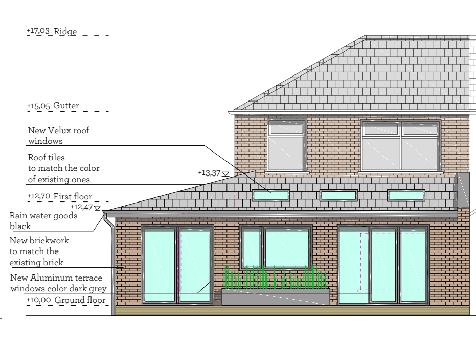
Garden elevation
