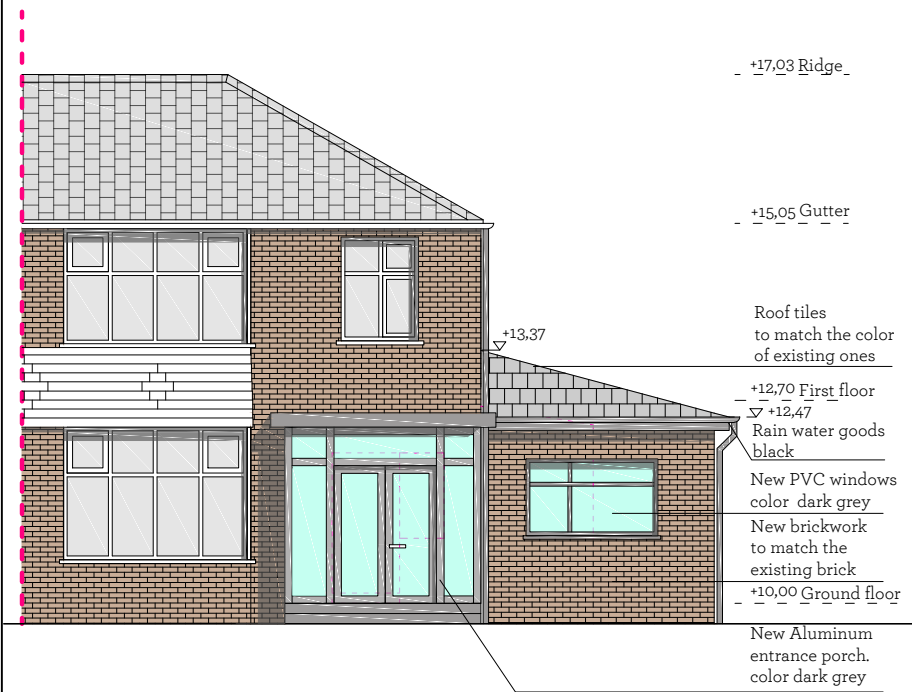
Front elevation
