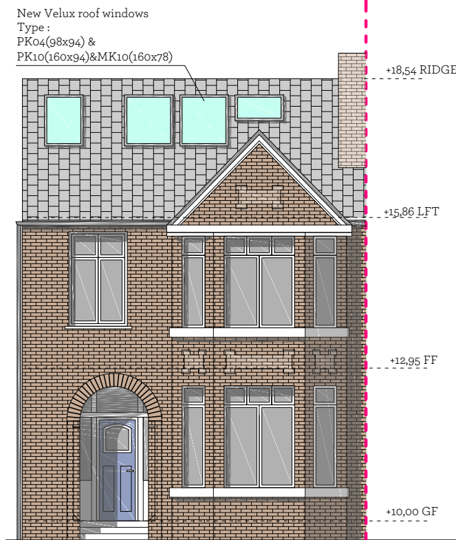
Front elevation
