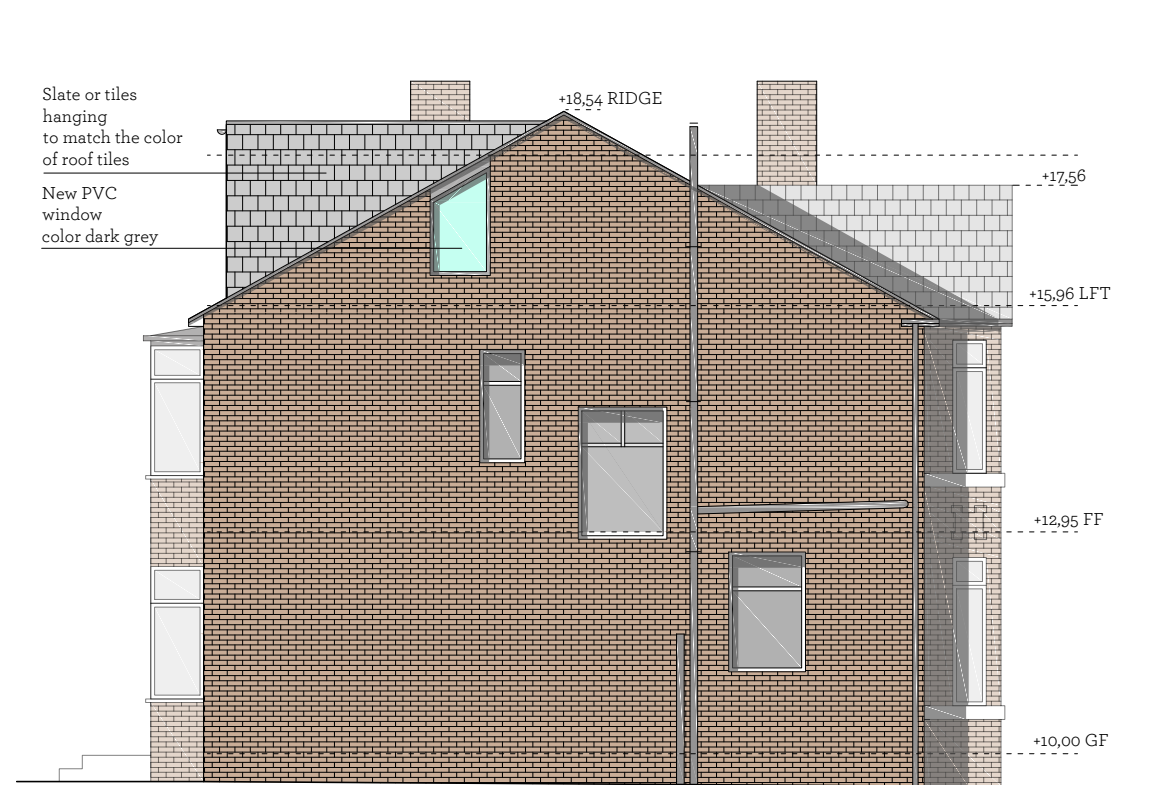
Side elevation
