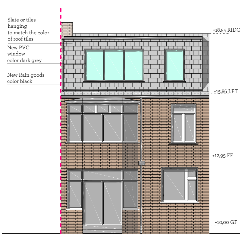
Garden elevation
