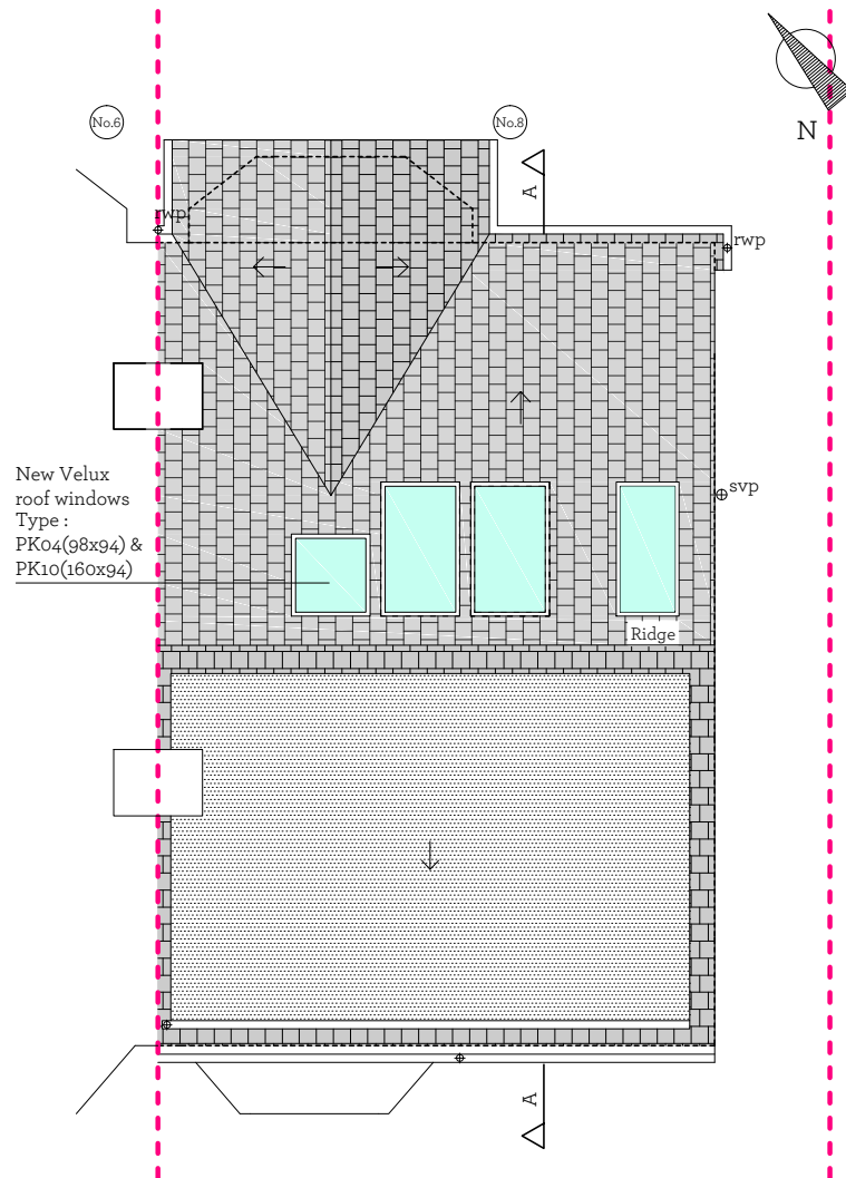
Roof Plan
