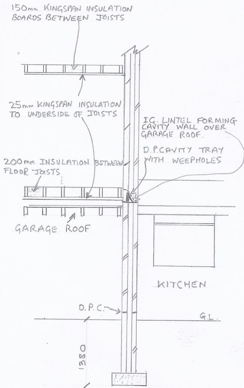
SECTION B:B
