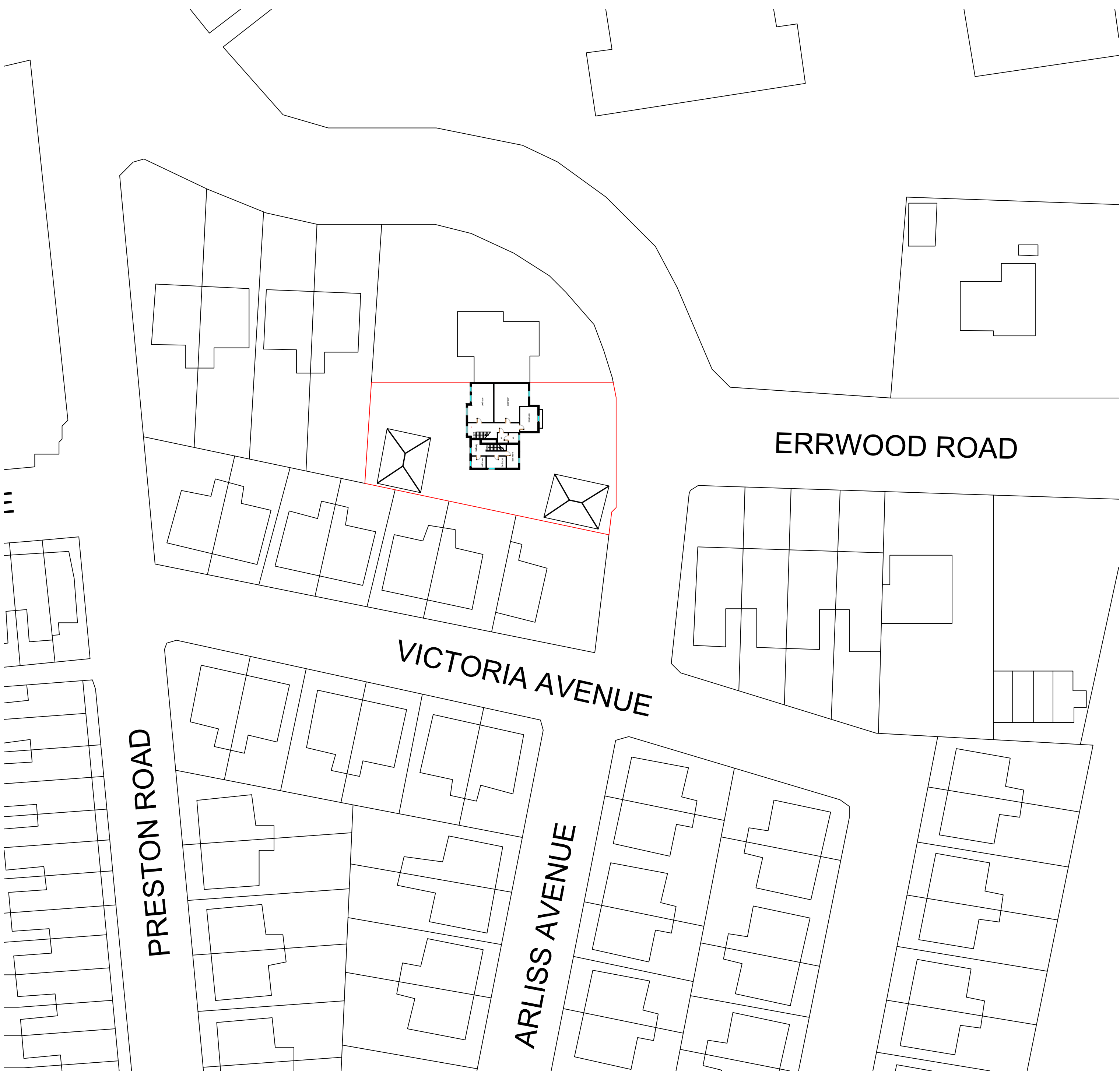
PROPOSED BLOCK PLAN 1:500 @ A1
