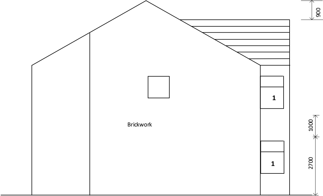
PROPOSED SIDE ELEVATION (H. No. 63)
