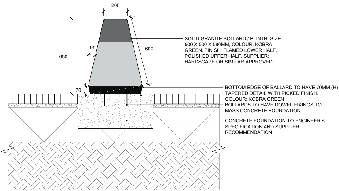
03B BESPOKE GRANITE CUBE / BOLLARD 602 SECTION
