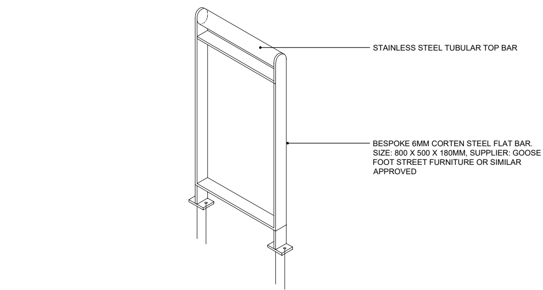
02C CYCLE STAND 602 ISOMETRIC
