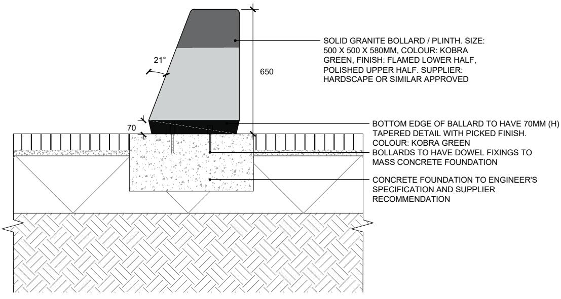
03C BESPOKE GRANITE CUBE / BOLLARD 602 SECTION
