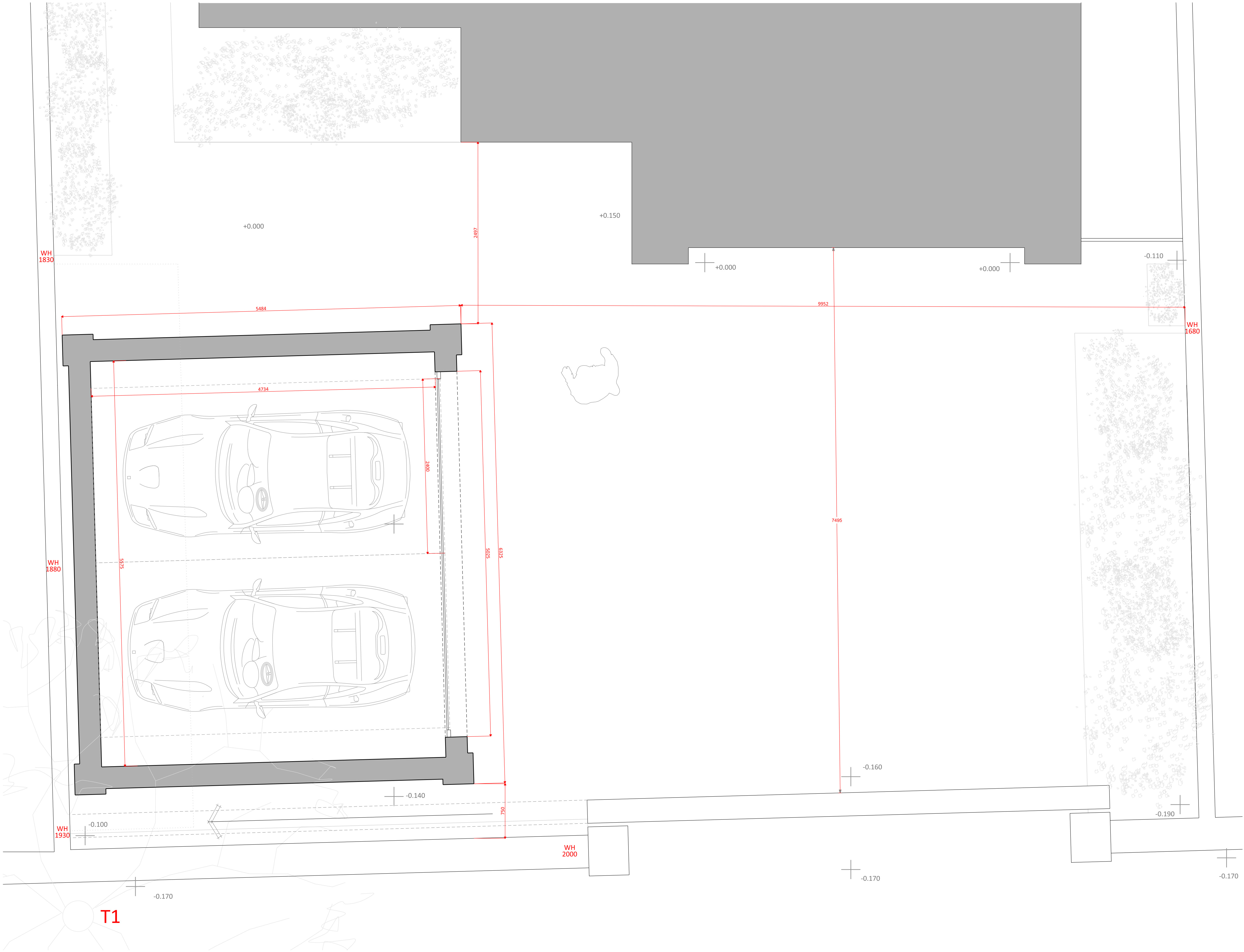
PROPOSED PLAN
