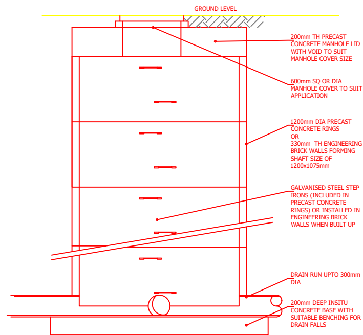
TYPICAL MANHOLE DETAIL FOR INVERT LEVELS >1.0m <3.0m DP
