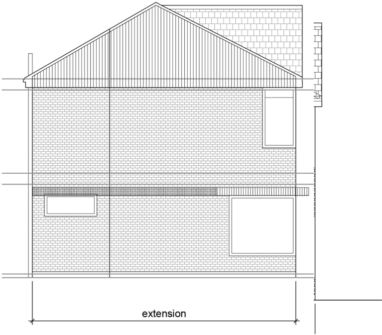
ELEVATION C
